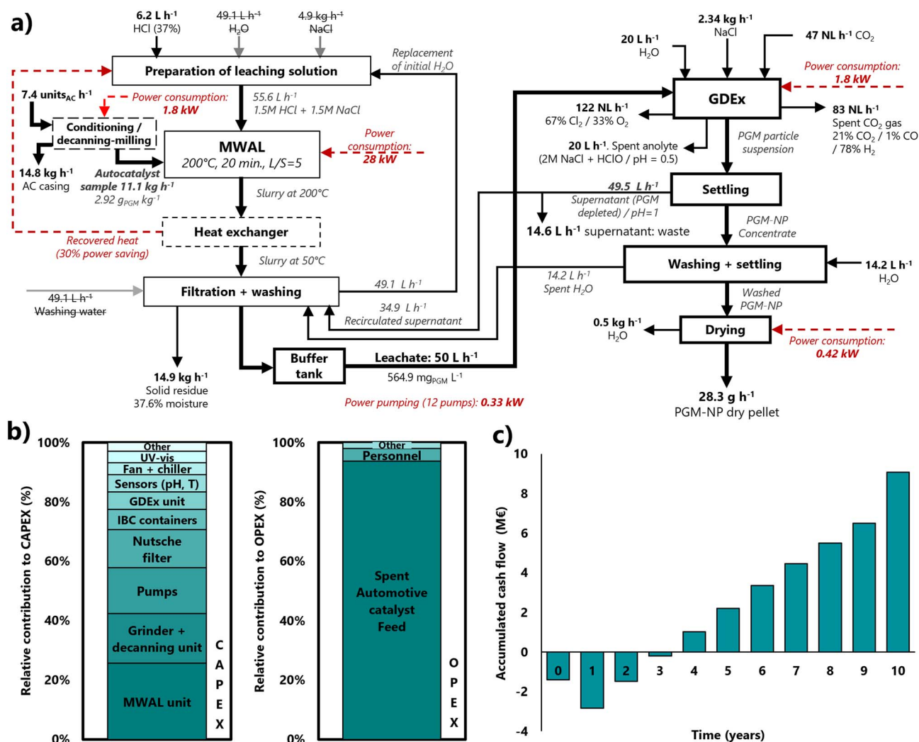
Fig. 5 Techno-economic performance of the integrated MWAL-GDEx process. (a) Mass and energy balance of the integrated process (MWAL operated at liquid-to-solid ratio, L/S ratio = 5; GDEx at 200 \text{ mA cm}^{-2} ). (b) Breakdown of the capital (CAPEX) and operational (OPEX) expenditures. (c) Cumulative cash flow and net present value (NPV) of the integrated process.
