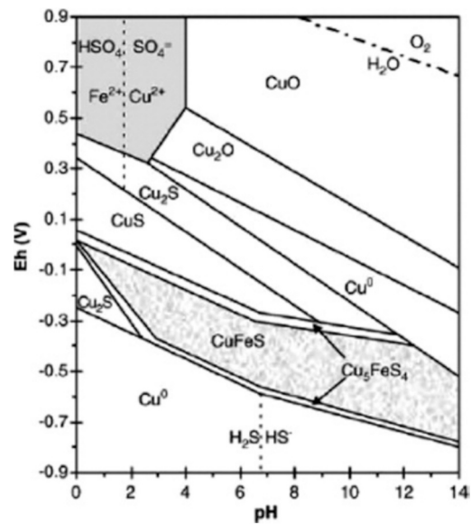
Fig. 4. Pourbaix diagram of Cu-Fe-S-H 2 O system at 25 °C (reproduced from Debernardi and Carlesi, 2013).
