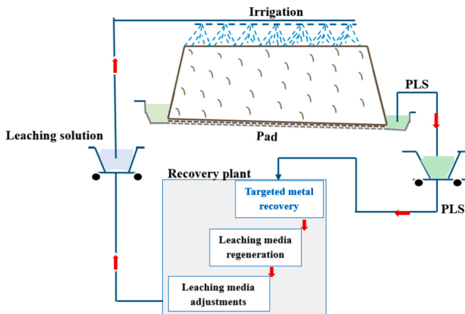
Fig. 1. Schematic of a typical copper sulphide heap leach circuit.
