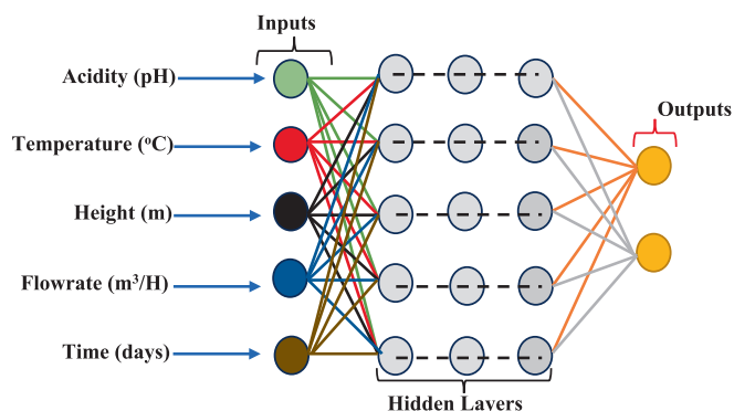
Fig. 5. Four layers ANN training prediction for metal recovery efficiency (structure (5–15–2):5: inputs, 15 neurons in hidden layers and 2 outputs).
