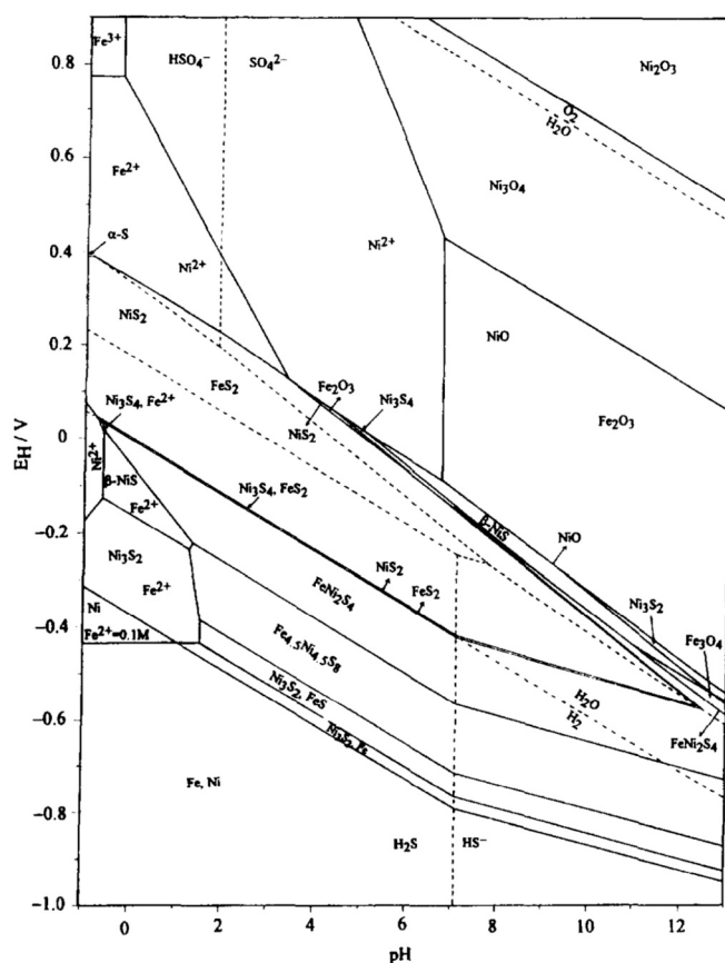
Fig. 3. Eh–pH diagram for Fe–Ni–S aqueous system at 298 K. Activities of aqueous sulphur (S), iron (Fe), and nickel (Ni) species = 0.1 mol/dm 3 . (reproduced from Warner et al., 1996 (Warner et al., 1996)).
