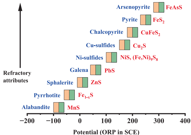
Fig. 2. Leaching potential of sulphide minerals.
