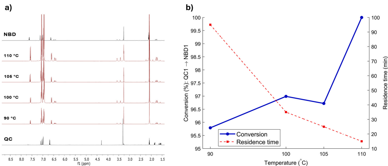
Fig. 10. a) ^1H NMR spectra (400 MHz, toluene- d_8 ) for QC1 (black line) and NBD1 (1.3 mol/L) solutions after photoisomerization at temperatures between 90 and 110 °C. b) Measured back conversion rates and residence times corresponding to the spectra shown in a). (For interpretation of the references to colour in this figure legend, the reader is referred to the web version of this article.)
