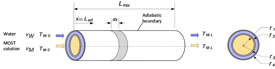
Fig. 8. Schematic of the heat exchanger and the corresponding geometrical and physical parameters.
