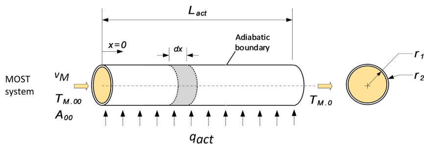
Fig. 7. Schematic of the activation component and the corresponding geometrical and physical parameters.
