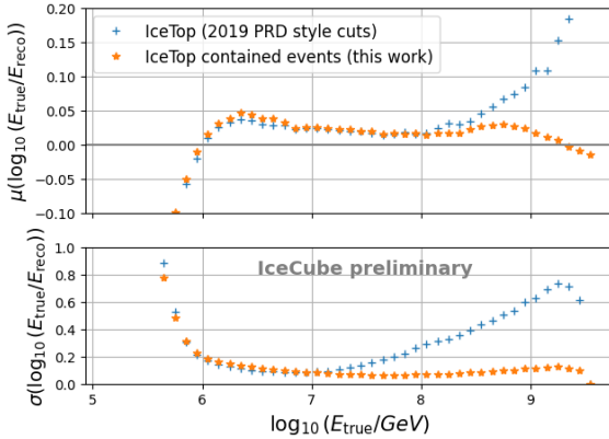
Figure 4: Comparison of the energy bias (top) and resolution (bottom) between the previous analysis in Ref. [2] and this work. Both show great improvements for the new cuts at the highest energies and similar performance for the lower energies. The slightly increased bias and resolution at the lowest energies are due to the increased zenith range.
