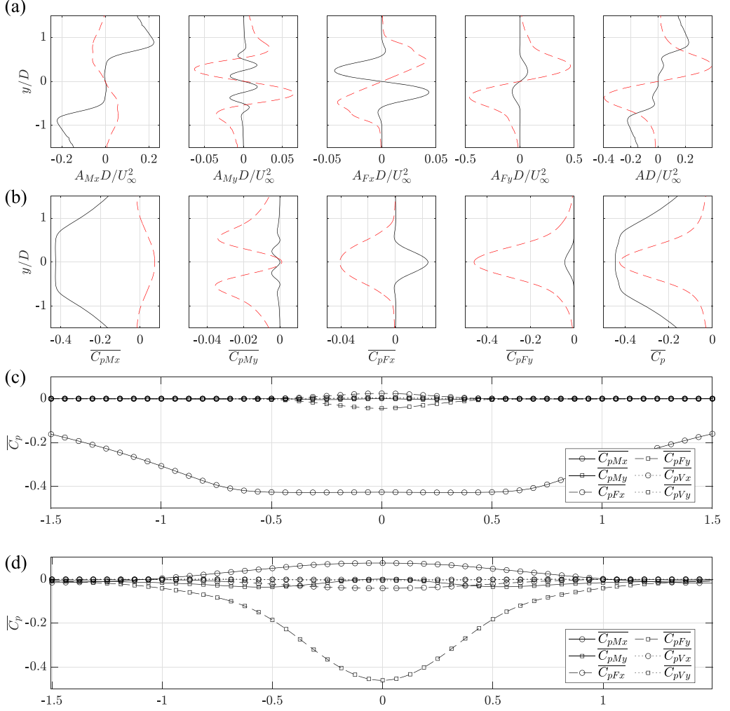
FIG. 7. (a) The distribution of each momentum budget at x/D = 1 (black solid curve) and x/D = 2.5 (red dashed curve), and (b) their integrated pressure. A comparison of the pressure contribution from each momentum budget for (c) x/D = 1 and (d) x/D = 2.5 .
