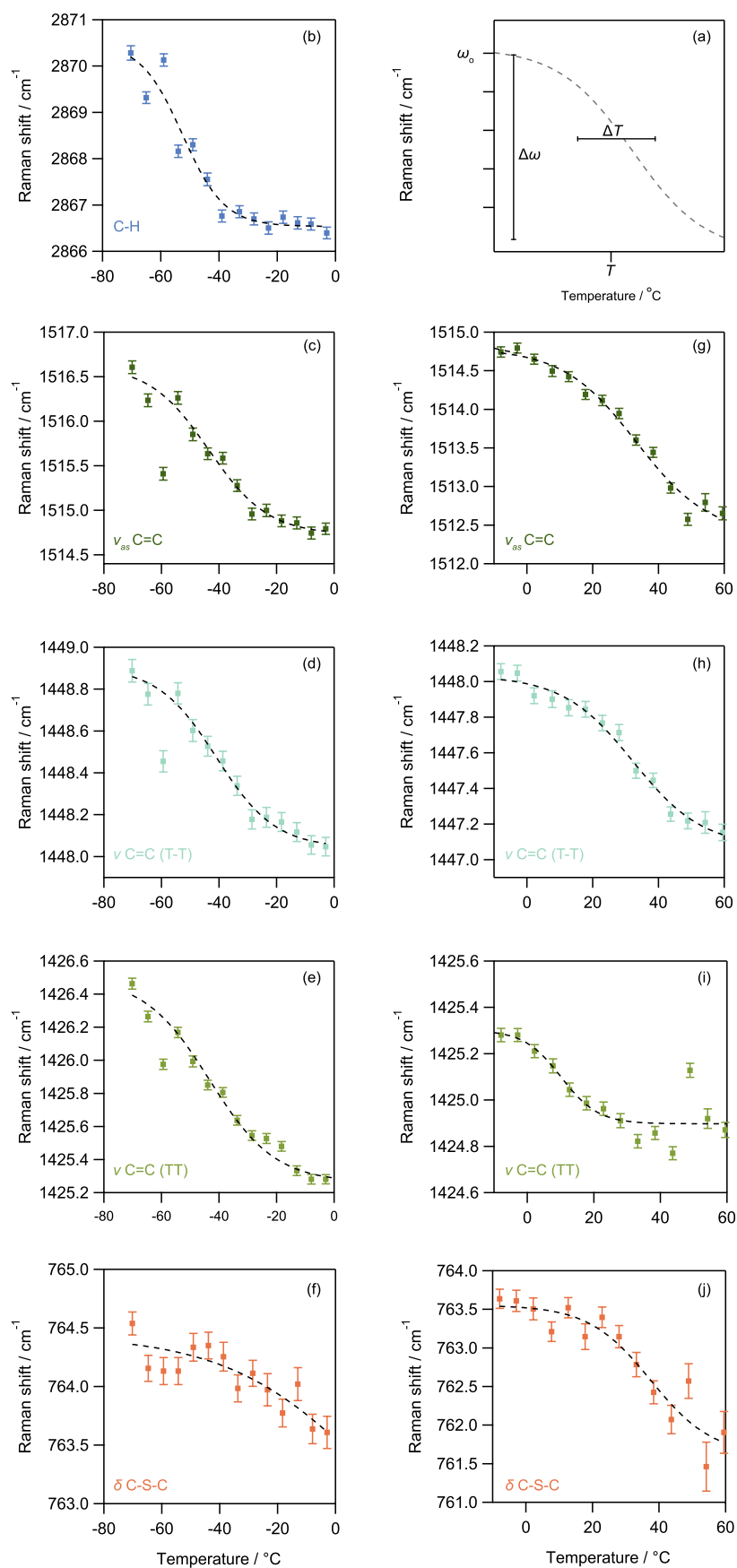
Figure 8. Raman shifts of selected vibrations as a function of temperature. (a) Dashed lines represent their fit by a sigmoid function. (b–f) The temperature region of the \beta -relaxation, (g–j) the temperature region of the \alpha -relaxation. The data point at -59.4 °C behaves as an outlier and was not included in the fitting with the sigmoid model.
