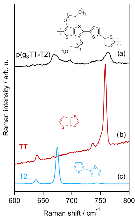
Figure 6. Raman spectra in the \delta\text{ C-S-C} region recorded at room temperature from (a) a p(g_3\text{TT-T2}) thin film, (b) TT, and (c) T2.
