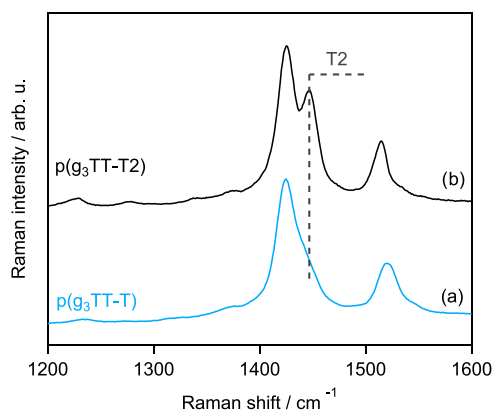
Figure 5. Raman spectra recorded at room temperature from thin films of (a) p(g_3\text{TT-T}) and (b) p(g_3\text{TT-T2}) .
