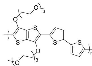
Figure 1. Molecular structure of the conjugated polymer p(g 3 TT-T2).
