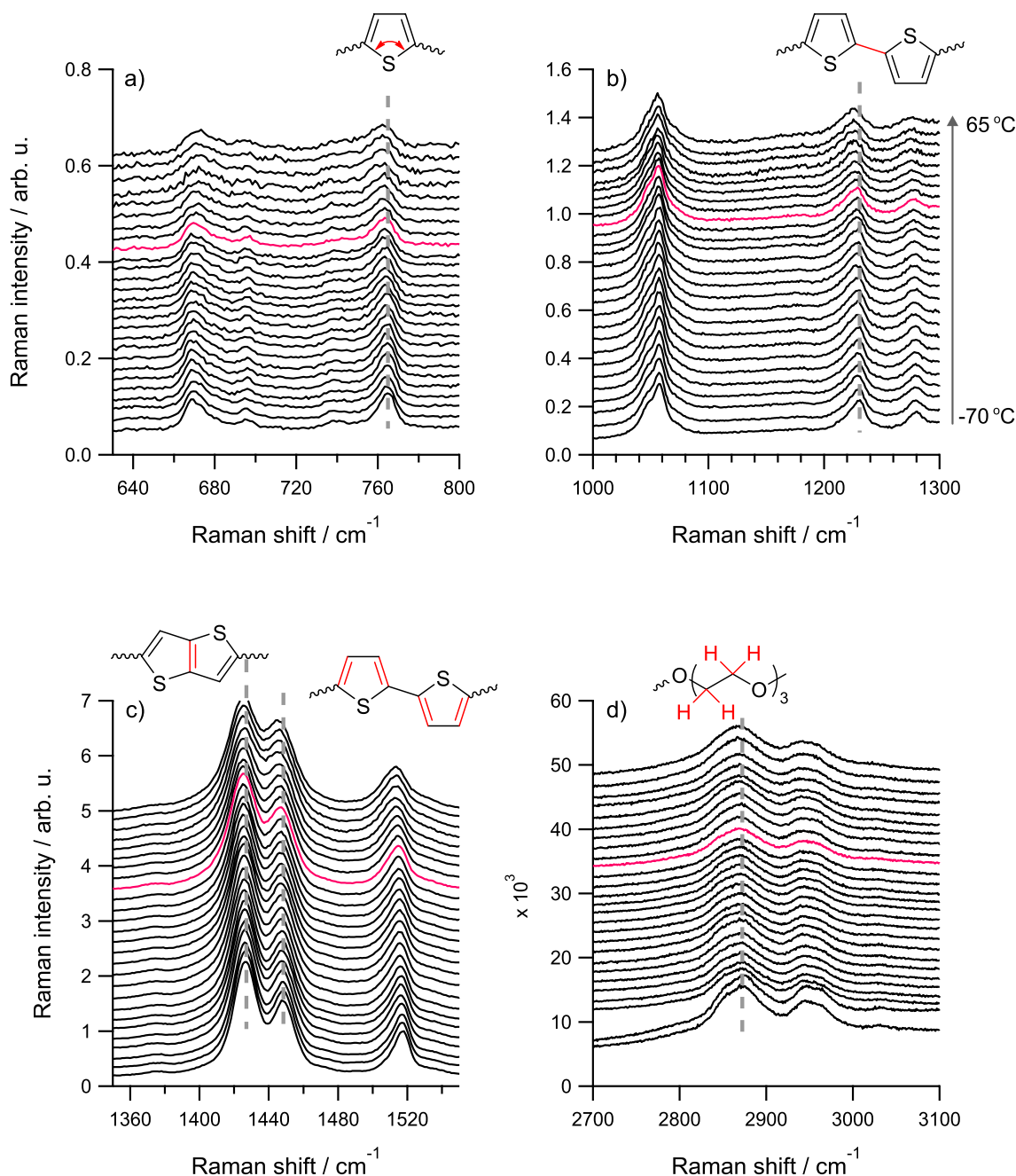
Figure 7. Temperature dependence of the Raman spectrum of p(g 3 TT-T2), recorded from -70 to 65 °C. Plots (a–d) show the close-up of different spectral regions, where particular vibrational modes appear. The traces in red are those recorded at room temperature.
