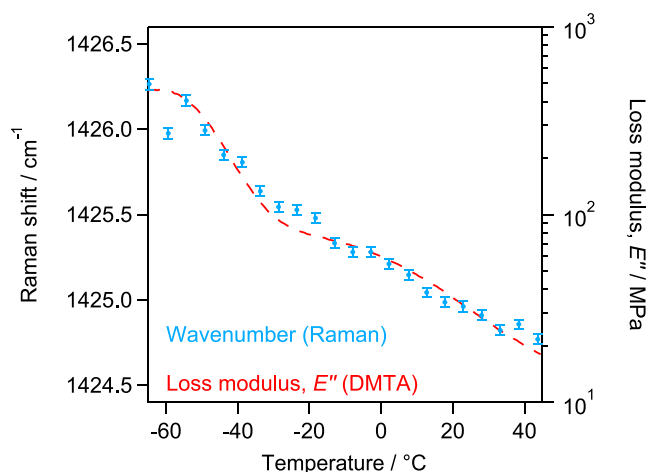
Figure 9. Temperature dependence of the Raman shift (left axis, blue dots, temperature scanned at 20 °C/min) and of the loss modulus ( E'' , right axis, dashed red line, measured at 1 Hz and temperature scanned at 15 °C/min), independently measured for p( g_3 TT-T2).
