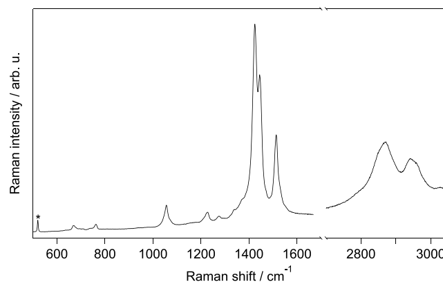
Figure 3. Raman spectrum of a thin film of p( \text{g}_3\text{TT-T2} ) recorded at room temperature. The asterisk marks the vibration at 520.6 \text{cm}^{-1} arising from the Si substrate onto which the thin film was deposited.
