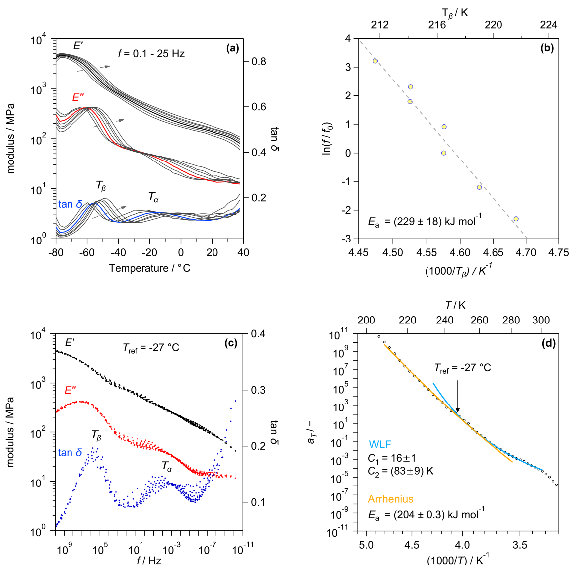
Figure 2. (a) Storage and loss moduli ( E' and E'' ) and loss tangent ( \tan \delta = E''/E' ) recorded by DMTA at frequencies ranging from f = 0.1 to 25 Hz (see direction of arrows; bold lines correspond to 1 Hz); (b) Arrhenius plot and linear fit (dashed line) of \tan \delta peak temperatures T_\beta associated with the \beta -relaxation process; (c) master curves for E' , E'' , and \tan \delta at T_{\text{ref}} = -27^\circ\text{C} ; and (d) DMTA frequency shift factors ( a_T ) such that E'(f, T) = E'(f_a, T_{\text{ref}}) , together with Arrhenius and Williams–Landel–Ferry (WLF) fits for T < T_{\text{ref}} and T > T_{\text{ref}} respectively.
