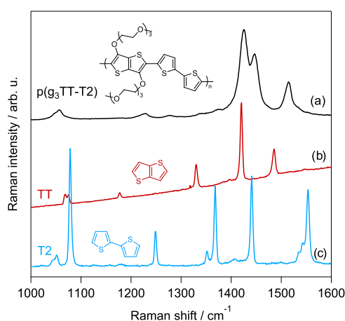
Figure 4. Raman spectra recorded at room temperature in the –C–C– and –C=C– stretching region for (a) a thin film of p(\text{g}_3\text{TT-T2}) , (b) thieno[3,2- b ]thiophene (TT), and (c) 2,2'-bithiophene (T2), the latter two as crystals. The molecular structure of each compound is also provided.
