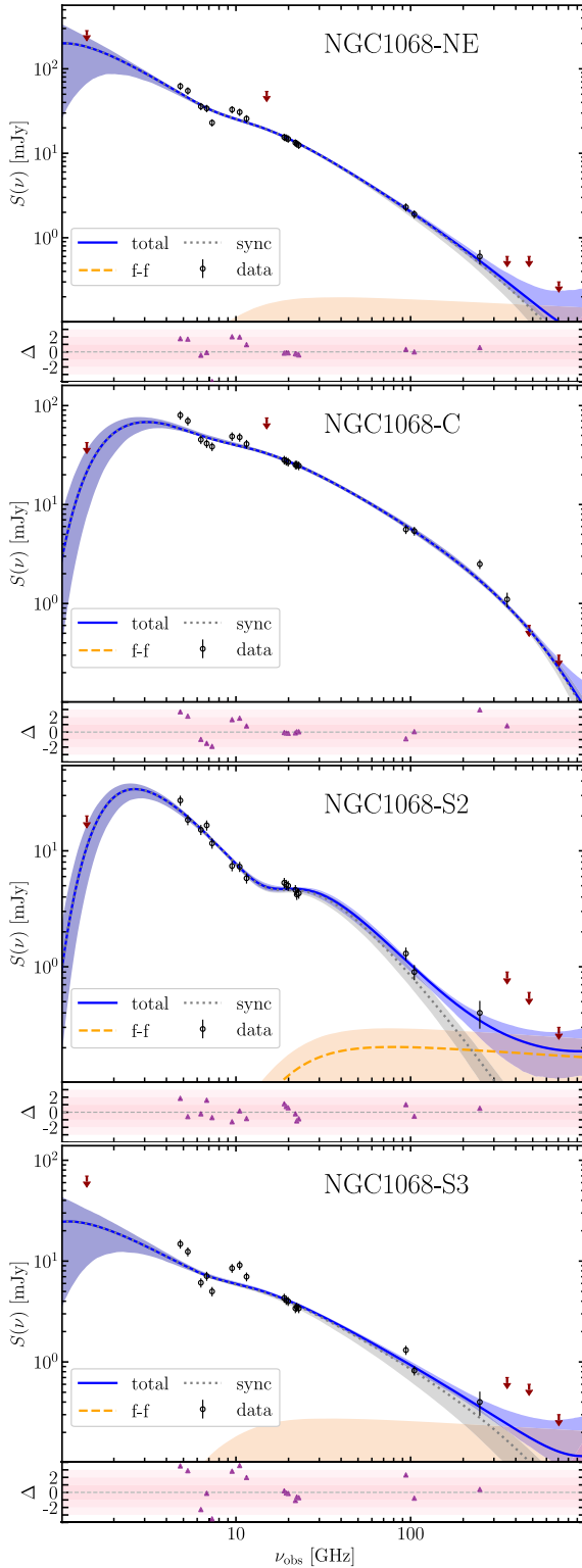
Figure 2. Matched-resolution cm-to-sub-mm SEDs of the compact jet components NE, C, S2, and S3. Circles are detections and arrows are upper limits. The solid blue curve is the posterior median total model, the grey dotted curve is the synchrotron contribution, and the orange dashed curve is the free-free contribution. The shaded regions show the 16th–84th percentile interval of the corresponding model component. The thermal-dust contribution is included in the fitting but is not shown because its upper limit is below the scale of the plots. The lower panels show the normalized residuals, \Delta = (S_{\text{obs}} - S_{\text{model}})/\sigma_{\text{obs}} .
