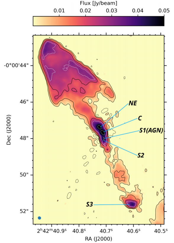
Figure 1. Composite e -MERLIN + VLA 4–12-GHz image of the inner radio jet in NGC 1068, showing the AGN component S1 and the compact off-nuclear components NE, C, S2, and S3. The image is reproduced in compact form from Mutie 2024; S1 is included here for morphological context and as the nearest potential contaminant of S2, but is not included in the off-nuclear SED fitting. This overview image is not used for the matched-resolution flux-density measurements.
