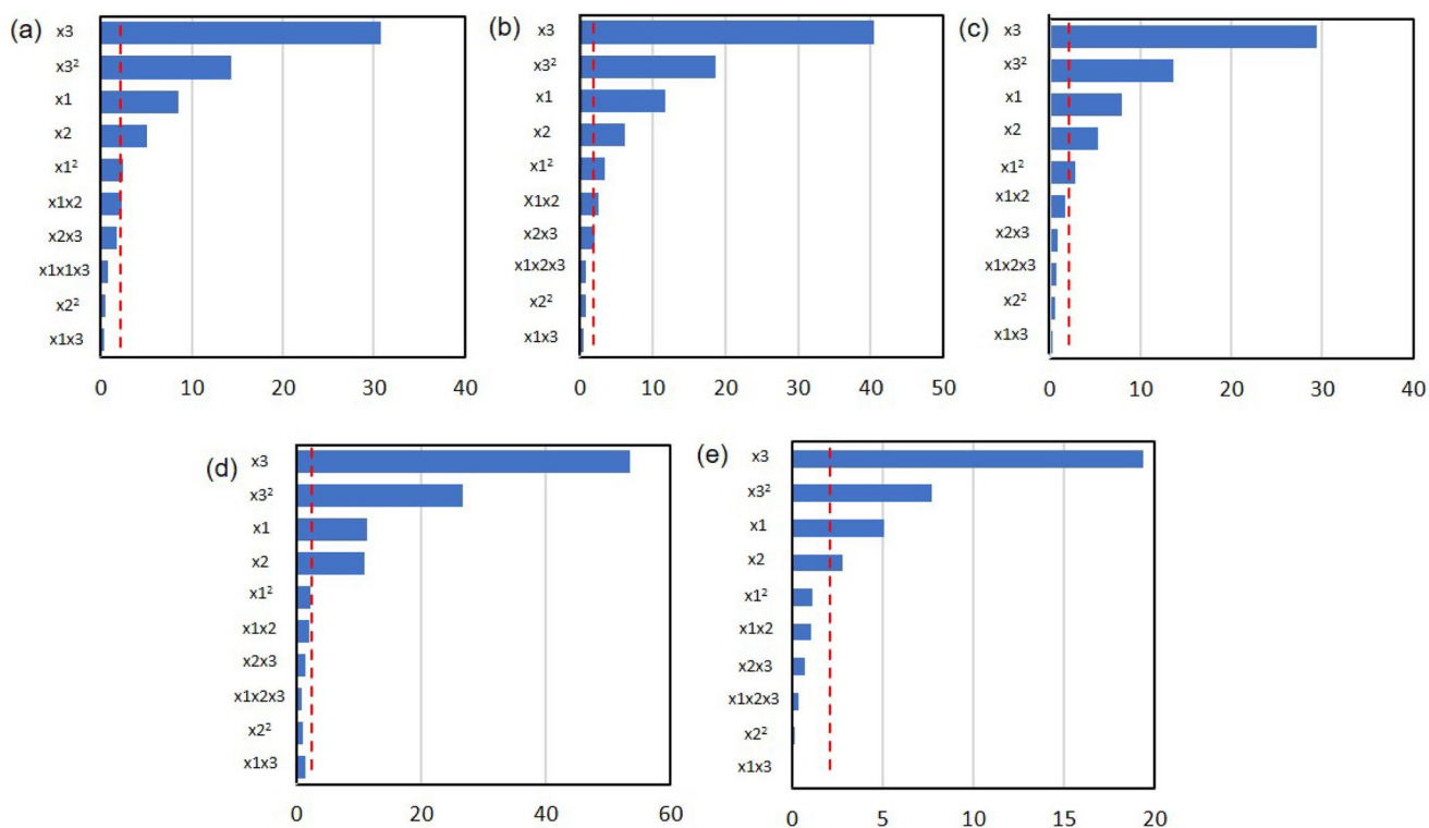
Fig. 10 Pareto charts of standardized effects for the regression models of a Nd, b Pr, c Dy, d Fe, and e B
