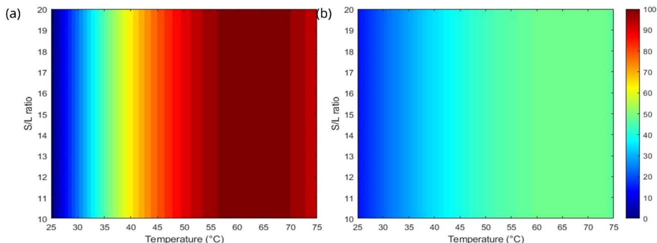
Fig. 5 Response surface plots of a Fe and b B
