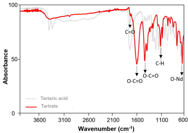
Fig. 3 FTIR spectrum of the leaching residue obtained after tartaric acid leaching of NdFeB magnets
