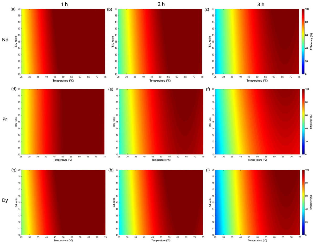
Fig. 4 Response surface plots for the leaching efficiency of Nd a 1 h, b 2 h, c 3 h; Pr d 1 h, e 2 h, f 3 h; Dy g 1 h, h 2 h, i 3 h
