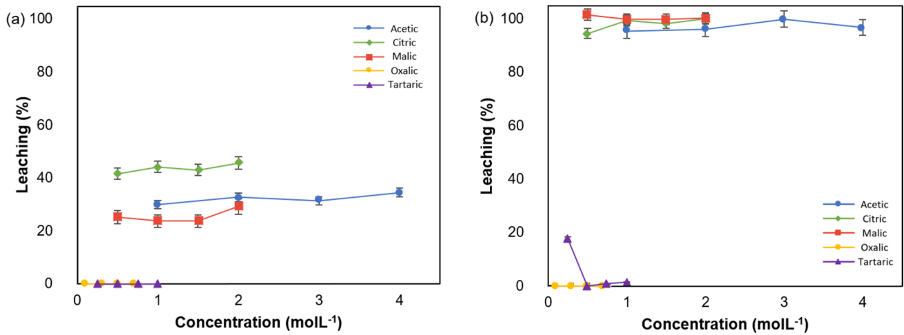
Fig. 2 Leaching of REE using organic acids as leaching agents for a 2 h and b 24 h (S/L ratio of 1/30 at 25 °C)
