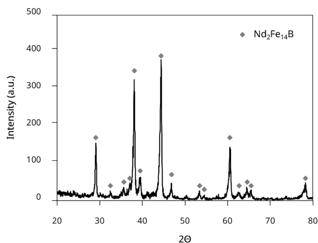
Fig. 1 REE magnet X-ray diffraction pattern after demagnetization
