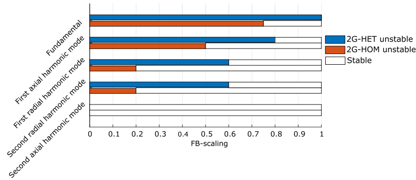
Fig. 9. Stability of each mode as a function of the FB-Scaling. Comparison between 2G-HET (blue) and 2G-HOM (red).
