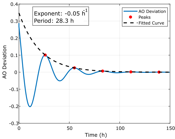
Fig. 4. Predicted change in axial offset as calculated by 2G-HET.
