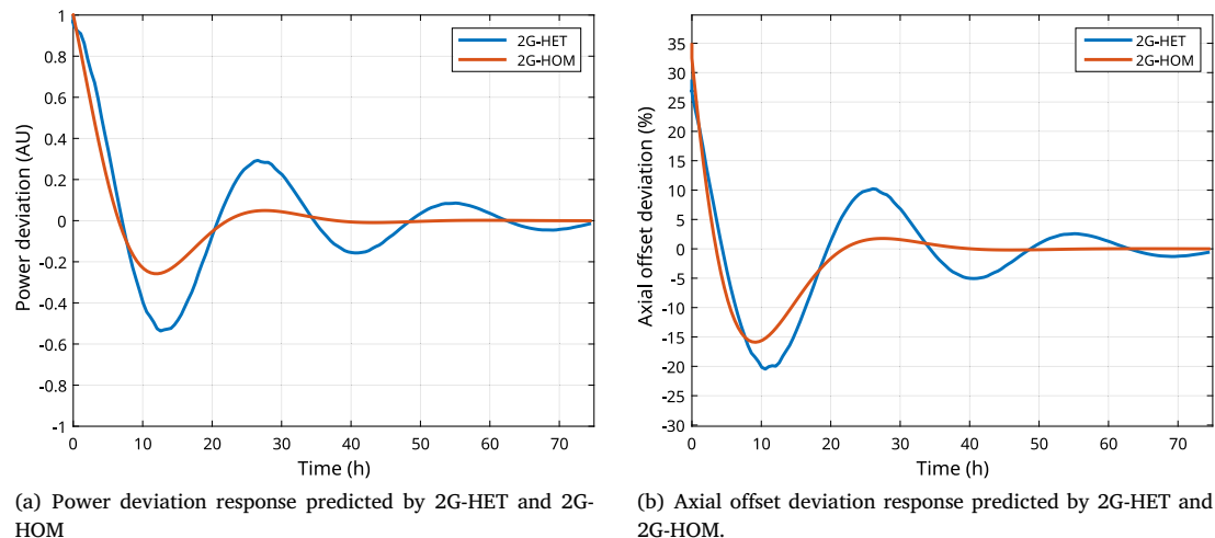
Fig. 15. Comparisons of power (left) and axial offset (right) between 2G-HET and 2G-HOM.
