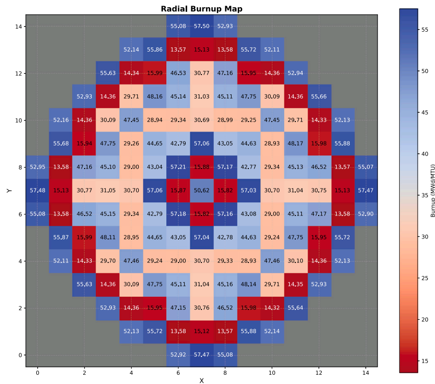
Fig. 1. Burnup map of the Ringhals-4 PWR reactor used in the case study.
