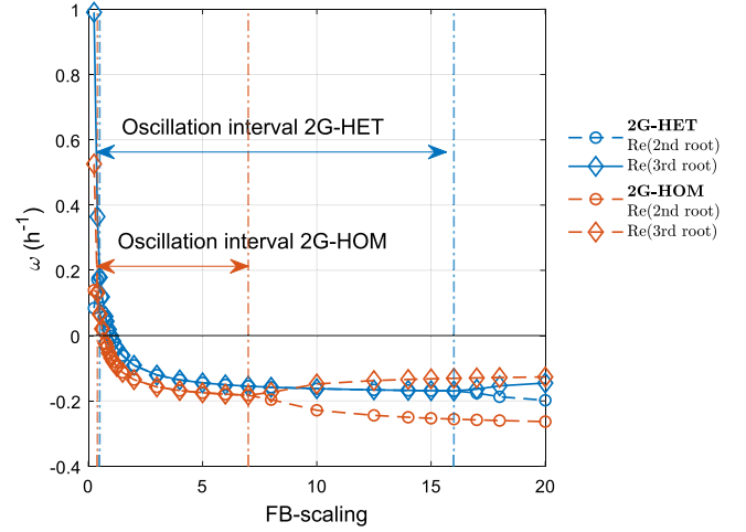
Fig. 8. Comparison of the analytically calculated stability coefficient between the 2G-HOM model and 2G-HET model. Dashed lines indicate the point of bifurcation of the stability coefficient.
