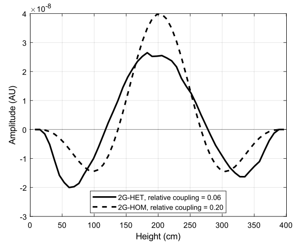
Fig. 12. Normalised axial profile of the coupling function P_{2,0,4} between the fundamental mode and the second axial harmonic mode compared between 2G-HET and 2G-HOM. “Relative coupling” in the legend refers to the integral of each of the profiles.
