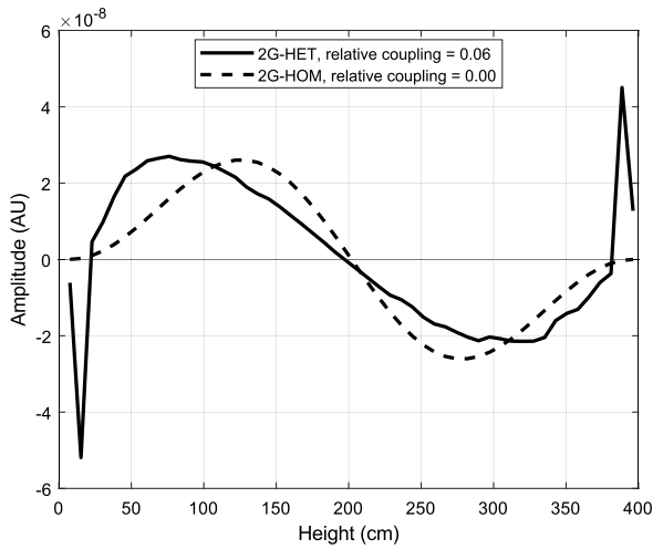
Fig. 13. Normalised axial profile of the coupling function FB_{0,1} between the fundamental mode and the first axial harmonic mode compared between 2G-HET and 2G-HOM. “Relative coupling” in the legend refers to the integral of each of the profiles.
