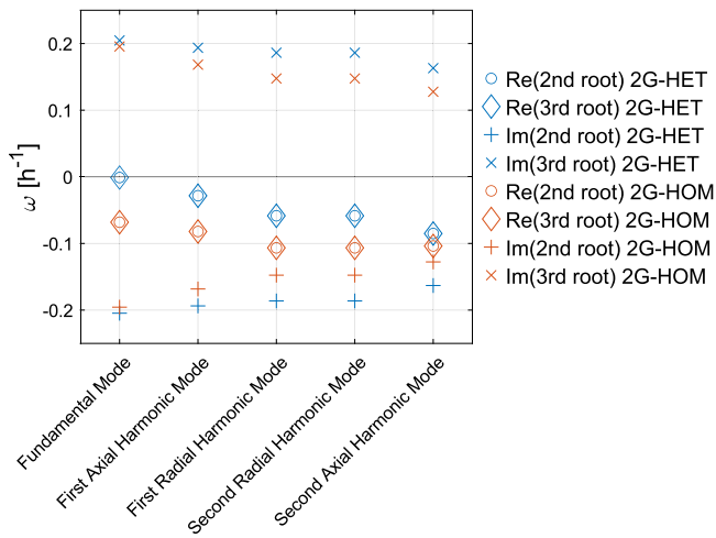
Fig. 10. Comparison of the modes of the real (circles and diamonds) and imaginary (crosses and plusses) parts of the second and third root of the 2G-HET (blue) and 2G-HOM (red). The real and imaginary values are equivalent to the stability coefficients and oscillation coefficients, respectively.
