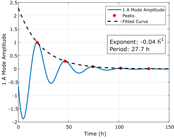
Fig. 7. Amplitude of the first axial harmonic mode of the neutron flux calculated by 2G-HET. “1 A Mode” refers to the first axial harmonic mode.
