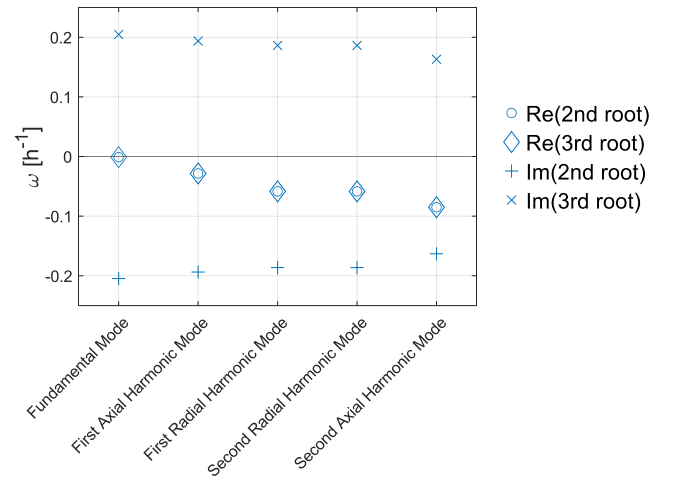
Fig. 5. Real (diamond and circle) and imaginary (crosses and plusses) parts of the second and third roots for each mode in 2G-HET. These real and imaginary values are equivalent to the stability and oscillation coefficients of the modes, respectively. The stability coefficient for the fundamental mode is negative.
