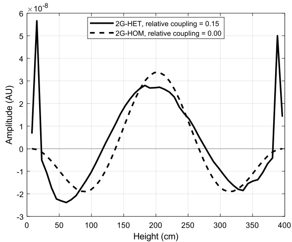
Fig. 14. Normalised axial profile of the coupling function FB_{0,4} between the fundamental mode and the second axial harmonic mode compared between 2G-HET and 2G-HOM. “Relative coupling” in the legend refers to the integral of each of the profiles.
