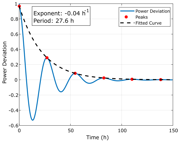
Fig. 3. Predicted change in power as calculated by 2G-HET.
