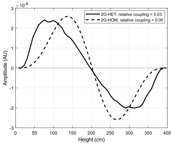
Fig. 11. Normalised axial profile of the coupling function P_{2,0,1} between the fundamental mode and first axial harmonic mode compared between 2G-HET and 2G-HOM. “Relative coupling” in the legend refers to the integral of each of the profiles.
