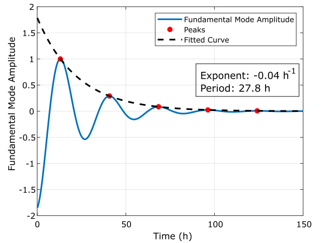
Fig. 6. Amplitude of the fundamental mode of the neutron flux calculated by 2G-HET.
