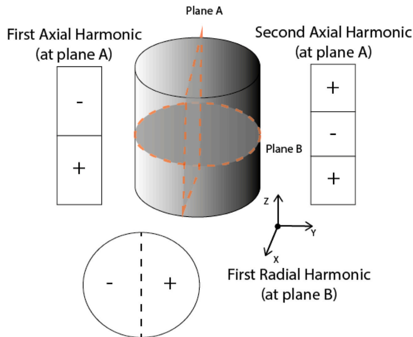
Fig. 2. Schematics of the first axial and radial harmonics and second axial harmonic of the system. The positive and negative deviations of the flux from its static value for the different modes are indicated by plus and minus signs, respectively. The orange dotted lines represent the axial and radial planes. Based on (Obaidurrahman and Singh, 2010).
