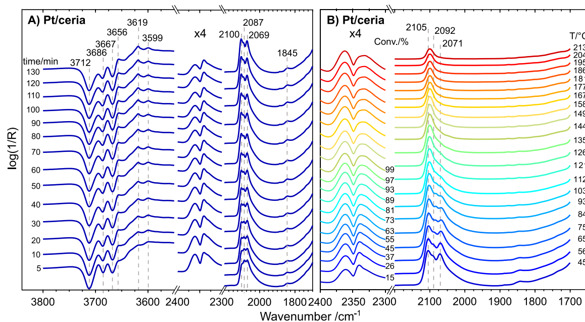
Fig. 6. Time-resolved infrared difference spectra collected in situ upon introduction of 0.2 vol.% CO and 1.0 vol.% O 2 (Ar as balance) at 35 °C to the Pt/ceria catalyst pre-exposed to 2.0 vol.% H 2 O for 2 h (panel A) and subsequent operando infrared difference spectra collected during increasing temperature (panel B).
