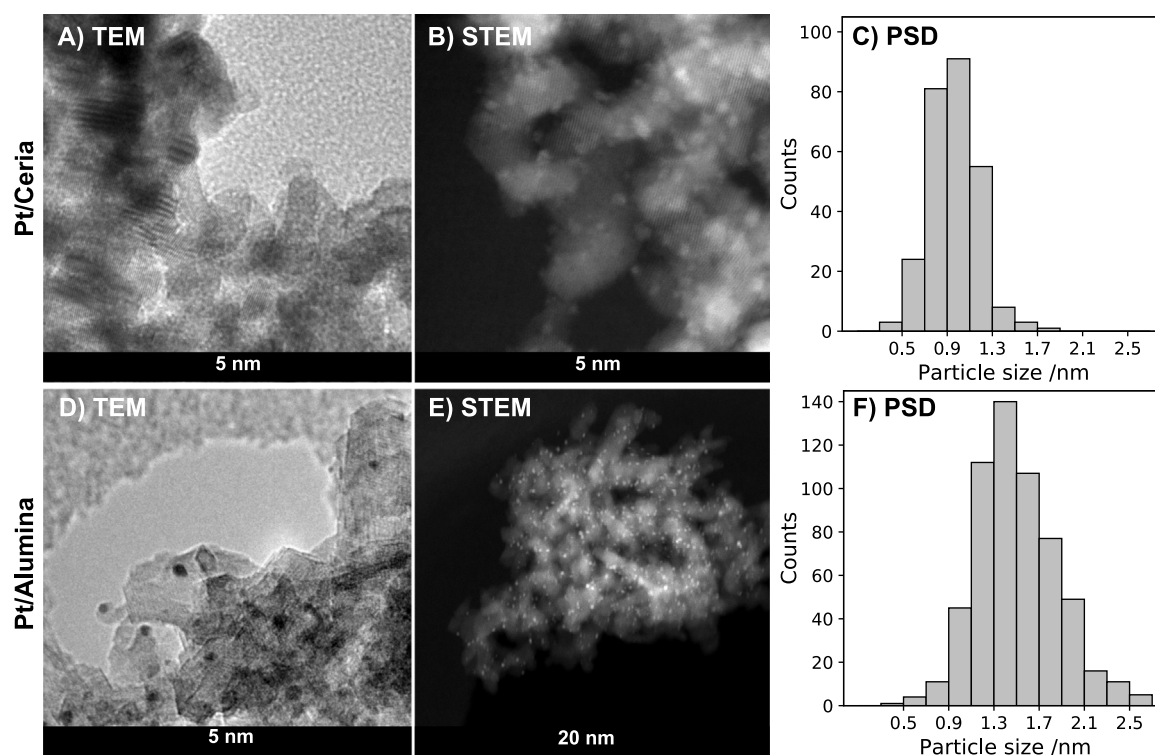
Fig. 2. High-resolution TEM (panel A) and STEM-HAADF (panel B) micrographs as well as platinum particle size distribution (panel C) of the spent Pt/ceria catalyst. Panels D-F show the corresponding results for the spent Pt/alumina. For the spent Pt/ceria catalyst, the average platinum particle size is 1.1 nm based on 265 Pt particles and for Pt/alumina catalyst the corresponding average size is 1.6 nm based on 585 particles.
