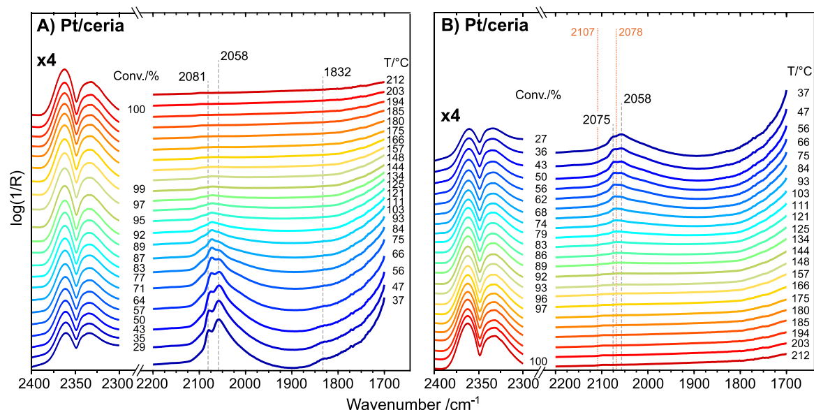
Fig. 4. Operando infrared difference spectra (hydrogen treated sample as reference) collected at indicated sample temperatures while increasing (panel A) and decreasing (panel B) the sample temperature in steps in the presence of 0.2 vol.% CO, 1 vol.% O 2 and 2 vol.% H 2 O (Ar as balance). The measured global CO conversion is indicated at each temperature. The vertical orange dashed lines in panel B indicate peak positions previously observed in dry conditions [15].
