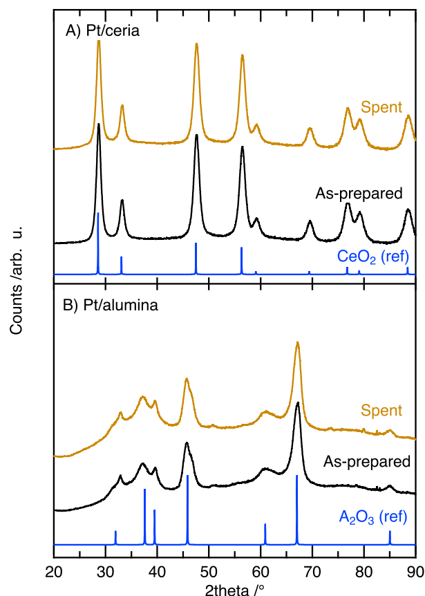
Fig. 1. XRD patterns of the as-prepared and spent, i.e., after dry and wet CO oxidation, Pt/ceria (panel A) and Pt/alumina (panel B) catalysts. The reflections are assigned using reference patterns (blue) from the Powder Diffraction File™ (PDF) database for cubic \text{CeO}_2 (PDF 00-004-0593) and \gamma - \text{Al}_2\text{O}_3 (PDF 00-010-0425).
