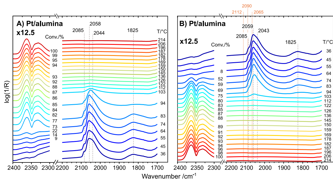
Fig. 5. Operando infrared difference spectra (hydrogen treated sample as reference) collected at indicated sample temperatures while increasing (panel A) and decreasing (panel B) the sample temperature in steps in the presence of 0.2 vol.% CO, 1 vol.% O 2 and 2 vol.% H 2 O (Ar as balance). The measured global CO conversion is indicated at each temperature. The vertical orange dashed lines in panel B indicate peak positions previously observed in dry conditions [15].
