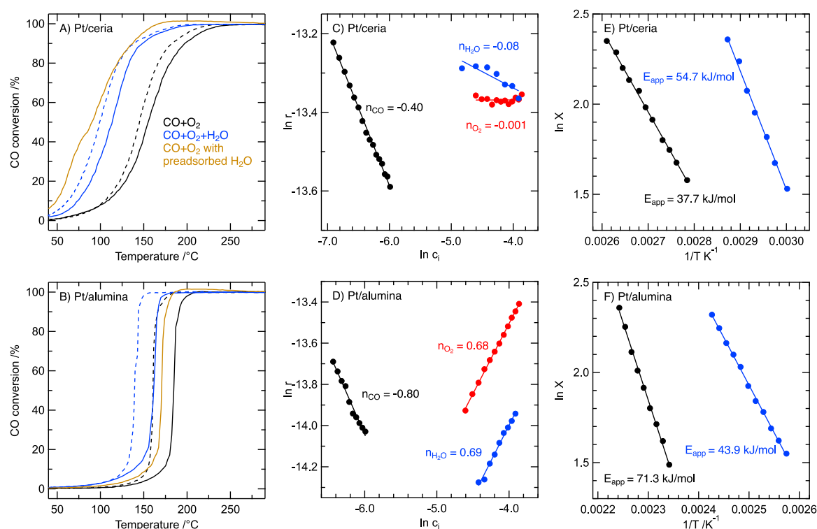
Fig. 3. Panels A and B show ignition (solid lines) and extinction (dashed lines) profiles for dry CO oxidation with 0.2 vol.% CO and 1.0 vol.% O 2 (black), with the addition of 2.0 vol.% H 2 O (blue), and with pre-adsorbed H 2 O (brown). Panels C and D show CO, O 2 and H 2 O concentration dependencies of the CO oxidation reaction rate (mol CO 2 g -1 s -1 ) over Pt/ceria performed at 45 °C and Pt/alumina at 127 °C. Panels E and F show Arrhenius plots for dry (black) and wet (blue) CO oxidation conditions. The reaction orders and apparent activation energies were obtained by linear fitting of data obtained at low (< 10%) CO conversion whereof the latter was fitted to ignition data.
