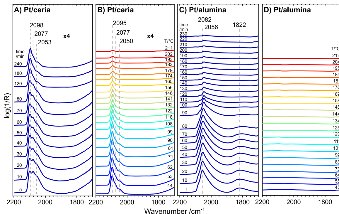
Fig. 7. In situ time-resolved infrared difference spectra collected at 35 °C upon introduction of 0.2% CO to the Pt/ceria (panel A) and Pt/alumina (panel C) catalysts that have been pre-exposed to H 2 O for 2 h. Subsequent in situ infrared difference spectra collected during a step-wise increase of the temperature in Ar flow for Pt/ceria (panel B) and Pt/alumina (panel D).
