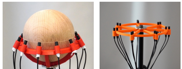
Figure 1: 5th-order EMA with pressure sensors and baffle, R = 40 mm (left), and 3rd-order EMA with virtual cardioid sensors and no baffle, R = 60 mm (right).
