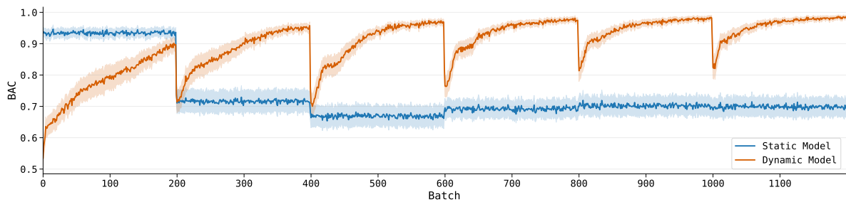
Fig. 4: Balanced Accuracy (BAC) over time for the static and dynamic attack detector, average and standard deviation from 100 experiment replications.
