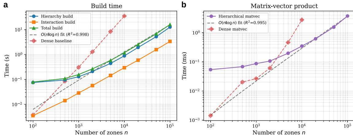
Figure 2 a) Build time vs. number of zones with O(n \log n) fit. b) Matvec time with dense baseline comparison.
