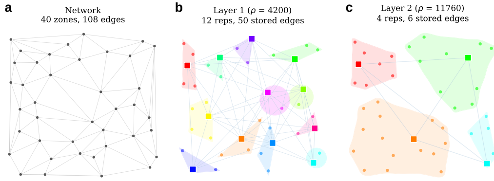
Figure 1 Hierarchy construction on a 40-zone random spatial network. a) Input graph. b) Layer 1 ( \rho = 4,200 ): 12 representatives (squares), each heading a group (shaded region). c) Layer 2 ( \rho = 11,760 ): 4 representatives with coarser groups. Stored edges connect representative pairs within the cutoff \alpha \cdot \rho_k .
