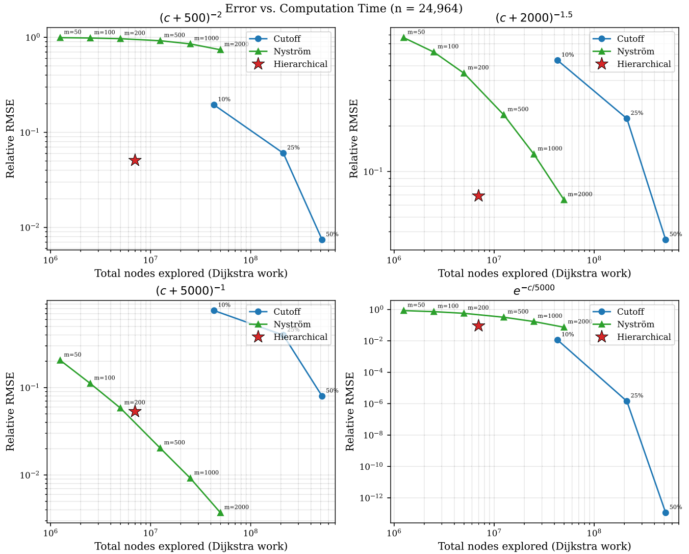
Figure 4 Error-vs.-computational-work Pareto frontier on a 25,000-zone grid network (spacing 1,000 m, diameter 314 km). The x-axis is total nodes explored (see text for definition); the y-axis is relative RMSE. Each panel corresponds to one interaction function. Cutoff variants are labeled by radius fraction of the network diameter; Nyström variants by landmark count m . The hierarchical operator (star) achieves competitive accuracy on steep kernels; on the smoothest kernel, Nyström dominates the error-work frontier.
