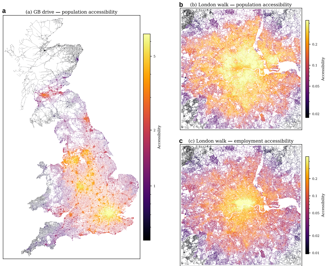
Figure 6 Accessibility maps computed by the hierarchical operator. a) Great Britain driving network ( n = 2,576,491 ): population-weighted accessibility with f(c) = (c + 300)^{-2} . b, c) London pedestrian network ( n = 1,765,539 ): population and employment accessibility with f(c) = (c + 60)^{-2} , walking speed 5 km/h. Edges are encoded by the mean accessibility of their endpoint nodes (log scale, per-panel normalization). Activity vectors are Census counts disaggregated to buildings by floor area. Each hierarchy is built once; subsequent matvec evaluations take \sim 700 ms (GB) and \sim 150 ms (London). An interactive zoomable version is available at https://hierx.github.io/hierx-paper/interactive_maps/index.html . Network data © OpenStreetMap contributors, available under the Open Database License. Census data: Office for National Statistics and National Records of Scotland, Crown copyright, Open Government Licence v3.0.
