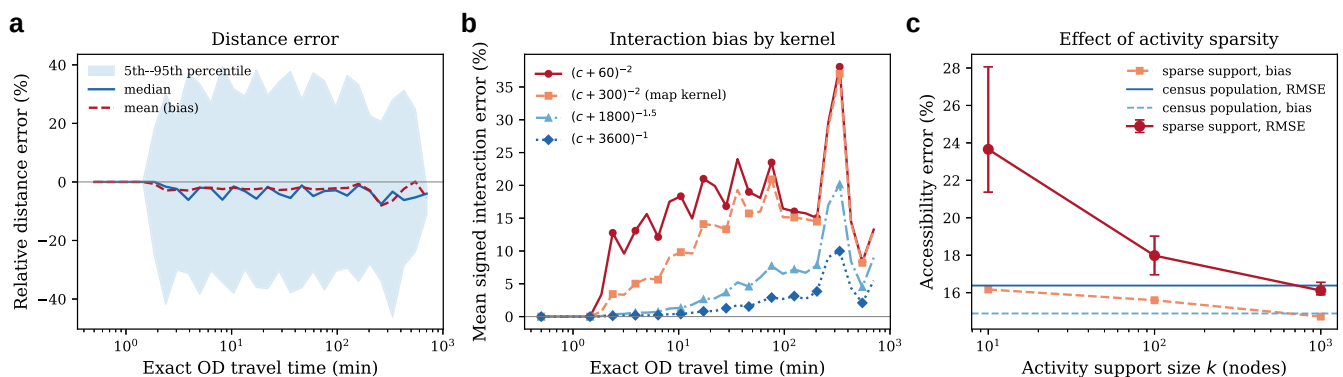
Figure 7 Error anatomy of the GB case study ( n = 2,576,491 , \alpha = 2 , \rho_0 = 60 s), against exact Dijkstra ground truth at 1,000 sampled origins. a) Relative distance error vs. exact OD travel time (536,656 sampled pairs): exact in the near field, then a nearly scale-free \sim 20\% spread with a small negative bias. b) Mean signed interaction error by distance bin for four kernels: convexity turns distance spread into systematically positive interaction bias, increasing with kernel steepness. c) Accessibility error vs. activity support size k (unit activity on k population-weighted nodes; exact full-network ground truth from k Dijkstra runs; whiskers span three trials): sparsity adds variance while the bias matches the census-population level (horizontal lines).
