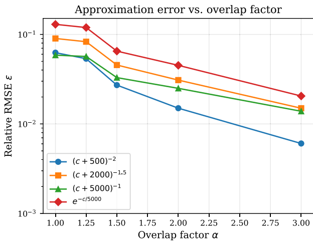
Figure 3 Relative RMSE \epsilon vs. overlap factor for four interaction functions ( 20 \times 20 grid, \gamma = 2 , \rho_0 = 4,000 m).
