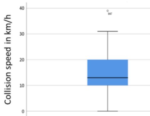
Fig. 5 Scenario 2, collision speed of truck in right turn crashes, based on GIDAS
