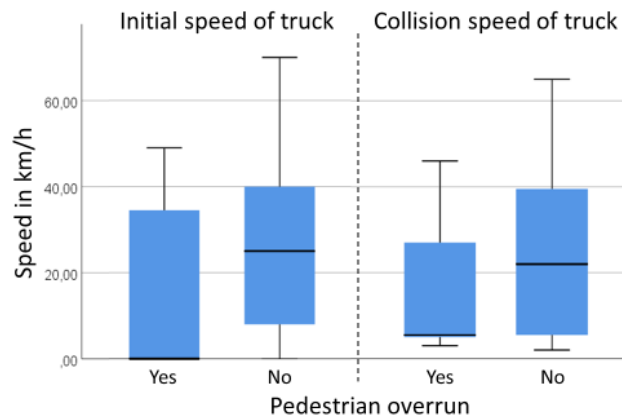
Fig. 7 Scenario 3, initial and collision speeds of truck in pedestrian crossing crashes, based on GIDAS
