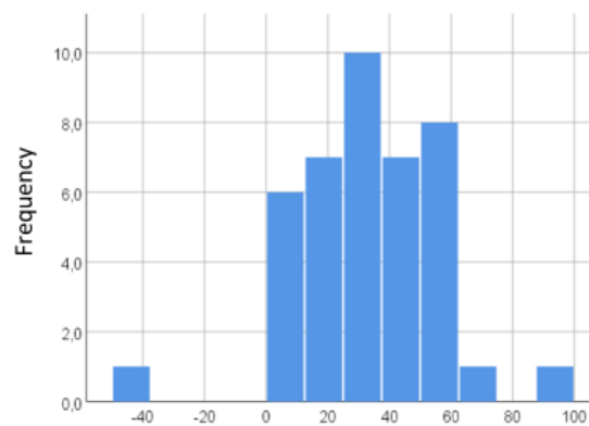
Fig. 6 Scenario 2, collision angles between truck and cyclist in right turn crashes, based on GIDAS
