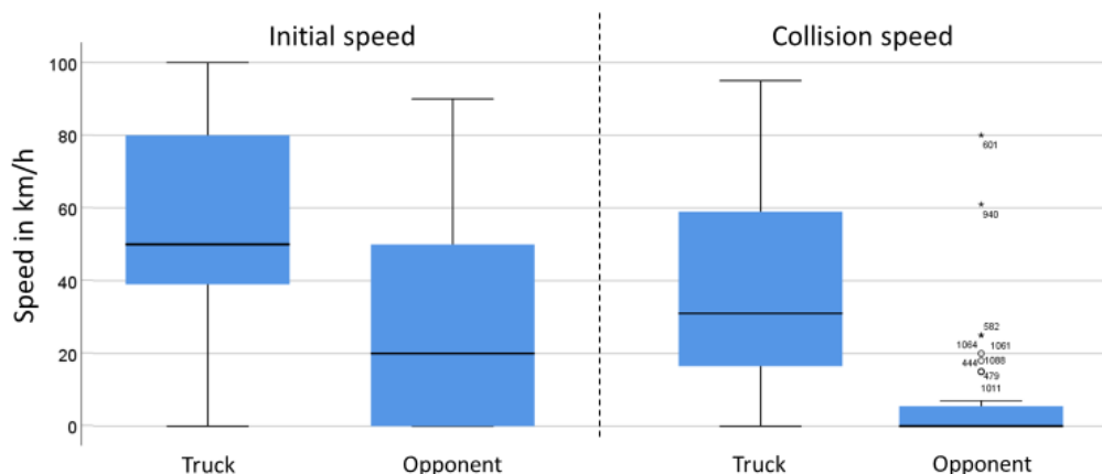
Fig. 4 Scenario 1, initial speeds of truck and collision partner in rear end crashes, based on GIDAS
