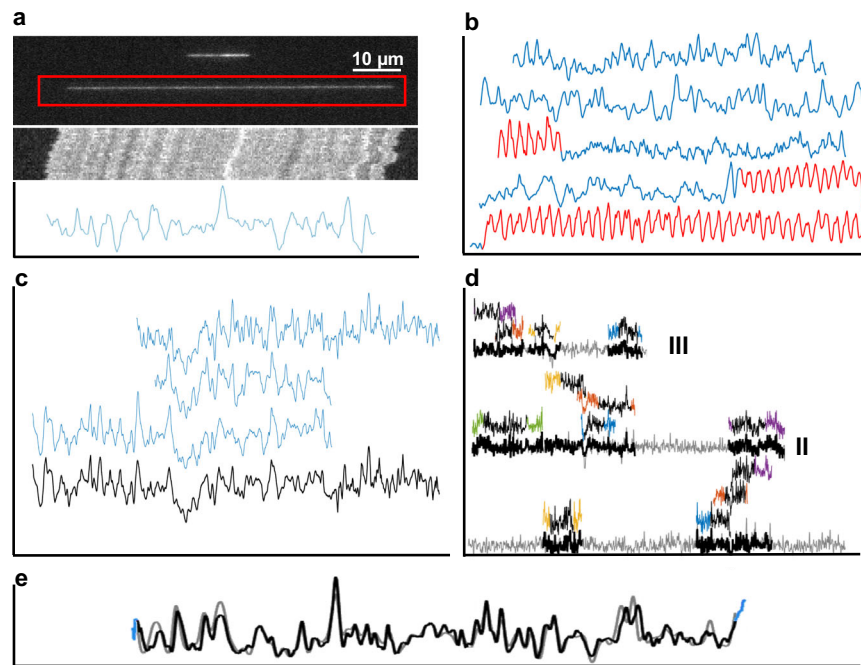
Fig. 1 | Workflow overview. a CB-labeled DNA molecules are stretched in nano-channels, imaged and detected (red box) to generate continuous fluorescence intensity profiles, referred to as barcodes. b Extracted barcodes undergo automated quality control and repetitive region (red) detection. c Multi-step assembly with the DOGMA pipeline generates barcode contigs (bargroups, black) from individual barcodes (blue). d Bargroups (colored) are aligned to reference genomes (gray) for reference-assisted refinement of unresolved joins, validation and
