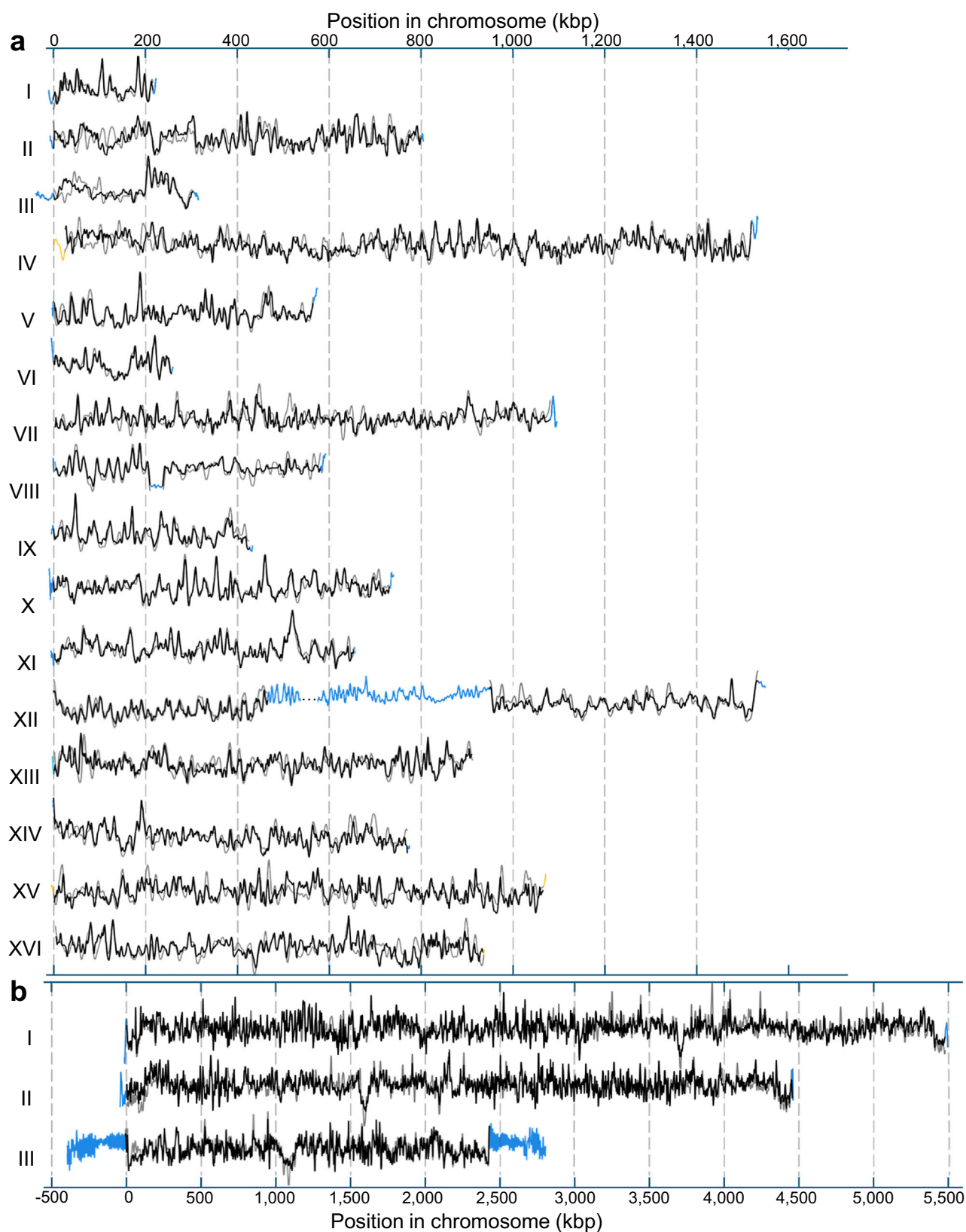
Fig. 5 | Full genome assemblies. a All assembled S. cerevisiae chromosomes (black) aligned to the reference (gray). b All assembled S. pombe chromosomes (black) aligned to the reference (gray). Chromosomal extensions relative to the reference
