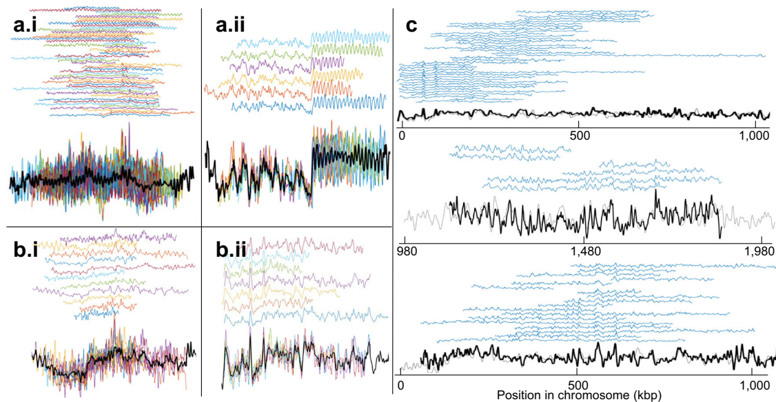
Fig. 4 | Assembly of bargroups. Example bargroup assembled a.i without masking and a.ii after masking of repetitive regions. Constituent barcodes are shown in color and the resulting bargroup consensus in black. Note that the repeat-masking procedure makes it so that the bargroups shown in these examples are assembled from different initial conditions and therefore do not contain the same constituent barcodes. b Examples of bargroups illustrating different signal-to-noise (SNR) characteristics. b.i A bargroup that fails (SNR = 0.9) the SNR criterion and b.ii a
