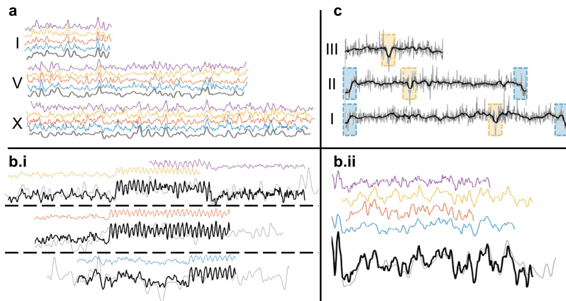
Fig. 3 | Considerations for dense OGM assembly of eukaryotic genomes. a Representative barcodes (colored) spanning entire reference chromosomes (gray) in S. cerevisiae . Examples of the same partially repetitive barcodes (colored) aligned to the reference genome (gray) before ( b.i ) and after ( b.ii ) masking of repetitive regions. Corresponding barcodes have the same color in both panels. The consensus barcode of each alignment is shown in black for comparison.
