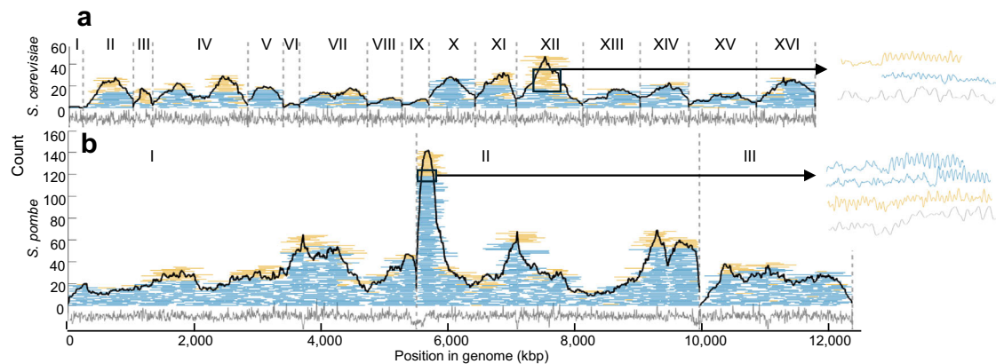
Fig. 2 | Alignment to reference genomes. Alignment of all barcodes ( N = 1653 ) to the reference genomes of a S. cerevisiae BY4742 and b S. pombe 972h-, with chromosomes indicated as Roman numerals. Matches to the correct species are represented in blue and to the incorrect species in yellow. The theoretical optical
