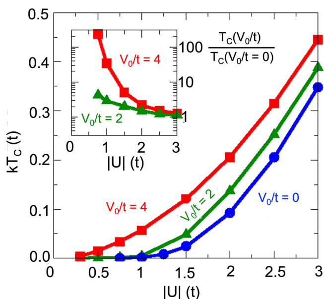
Fig. 2 | Critical temperature T_c in the presence of a superpotential V_0 . Comparison of T_c between homogeneous system ( V_0/t = 0 , blue) and in the presence of a superpotential with strength V_0/t = 2 (green) and V_0/t = 4 (red) where -t is the hopping between nearest-neighbors of the underlying square lattice. Results are shown as a function of the local attractive interaction U/t between electrons. Inset: Ratio between T_c with a finite superpotential and T_c for the homogeneous system. The solid red line in (e) is a fit to T_c/T_c^{hom} = \alpha|U|e^{\beta t/|U|} with the fitting parameters \alpha = 0.0436 and \beta = 6.663 as described in the text. We consider a charge concentration p = 0.5 .
