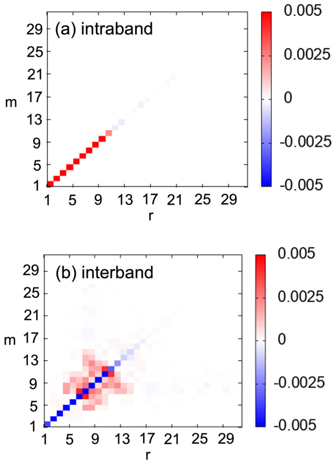
Fig. 5 | Intra- and interband contributions to the superfluid stiffness. Color surface plot of the contribution \mathcal{D}_{r,m} to the stiffness from transitions between bands r and m , see Eq. (5), divided into intraband r = m (a) and interband r \neq m (b) contributions. The model is a square lattice with hopping -t between nearest-neighbors and a local attractive interaction U/t = -2.0 between electrons. The strength of the imposed superpotential is V_0/t = 4 and we consider a charge concentration p = 0.5 .
