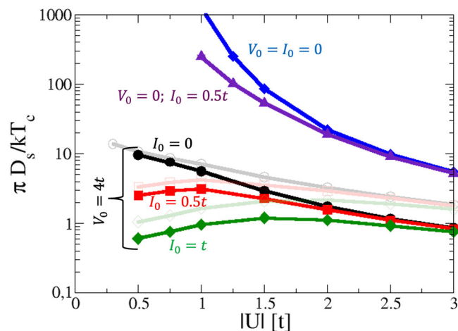
Fig. 6 | Ratio between the superfluid stiffness D_s and critical temperature T_c . The ratio is shown as a function of the local attractive interaction U/t between electrons where -t is the hopping between nearest-neighbors of the underlying square lattice (up to 24 \times 24 sites). Blue and violet curves are for the system without superpotential and impurity potentials I_0/t = 0.0 and I_0/t = 0.5 , respectively. In the presence of a superpotential ( V_0/t = 4 , patch size 4 \times 4 ) the results are shown for impurity strength I_0/t = 0 (black), I_0/t = 0.5 (red), I_0/t = 1 (green). Lines in the foreground (full symbols) and background (open symbols) refer to the random phase approximation (RPA) and mean-field (BCS) result, respectively. In case of V_0 = I_0 = 0 RPA and BCS result are identical, whereas for V_0 = 0 , I_0 = 0.5t the difference is within the size of the symbols. Charge density p = 0.5 .
