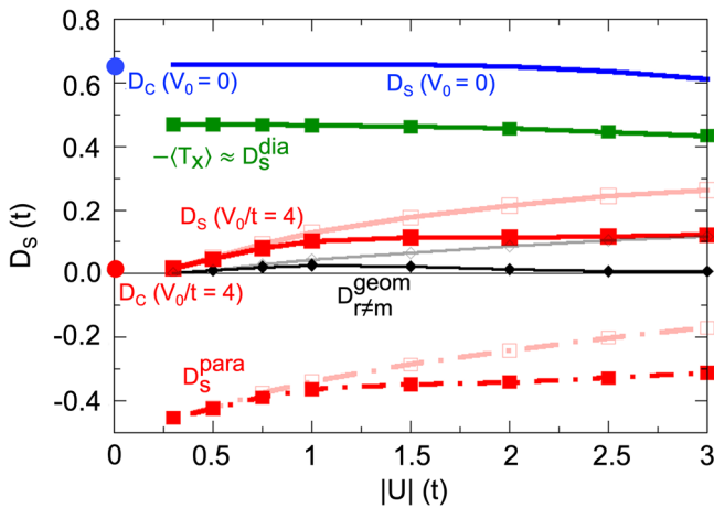
Fig. 4 | Impact of superpotential and gauge invariance on the superfluid stiffness. Superfluid stiffness D_{s,tot} for superpotential values V_0/t = 0 (blue) and V_0/t = 4 (red, squares) as a function of the local attractive interaction U/t between electrons where -t is the hopping between nearest-neighbors of the underlying square lattice. The stiffness is split into the diamagnetic (mostly intraband) ( D_s^{dia} ) and paramagnetic (mostly interband) ( D_s^{para} ) contribution. Also shown is the geometric contribution for r \neq m (black) which positively contributes to the stiffness. Lines in the foreground (full symbols) and in the background (open symbols) refer to the random phase approximation (RPA) and mean-field (BCS) result, respectively. For a vanishing attractive interaction U/t = 0 between electrons the charge stiffness D_c is shown by full circles while the superfluid stiffness D_s vanishes in this limit. Charge concentration: p = 0.5 .
