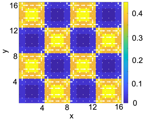
Fig. 3 | Current flow through the periodically modulated superconductor. Illustration of the gauge invariant superconducting current distribution (white arrows) for a vector potential applied along the x-direction. The local superconducting gaps are shown as colored background. The model is a square lattice with hopping -t between nearest-neighbors and a local attractive interaction U/t = -2.0 between electrons. The strength of the imposed superpotential is V_0/t = 4 and we consider a charge concentration p = 0.5 .
