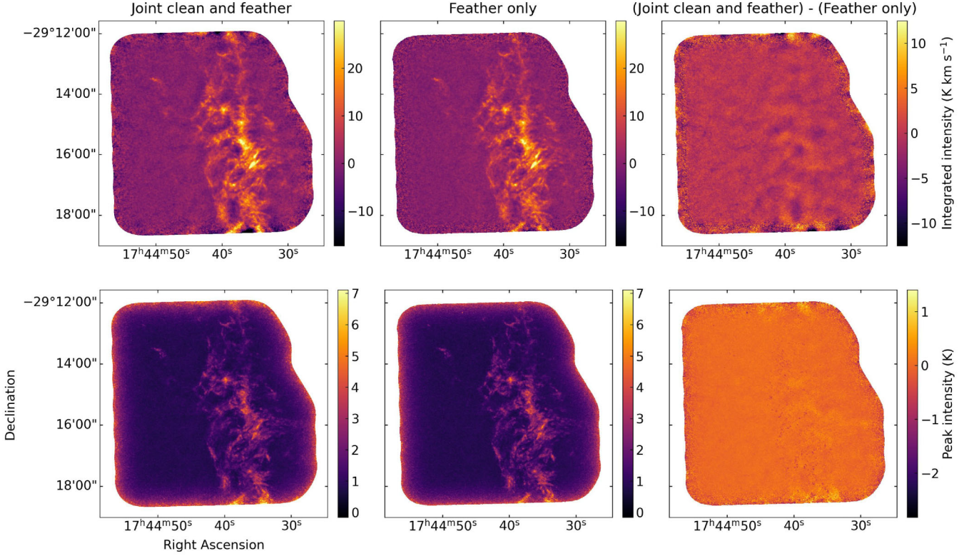
Figure 2. Comparison for field \tau between the two different array combination methods presented in Section 3.5. The top row shows integrated intensities over the subset of channels used for testing (see Fig. 3), while the bottom row shows peak intensities. The left column shows the results from the joint imaging of the 12 m and 7 m data, feathered with the TP data (Section 3.5.1). The central column shows the result from the feather only approach (Section 3.5.3). The right column shows the difference (joint clean and feather–feather only). Note that unlike the majority of figures in this paper, these are shown with Right Ascension and Declination to minimise unnecessary white-space.
