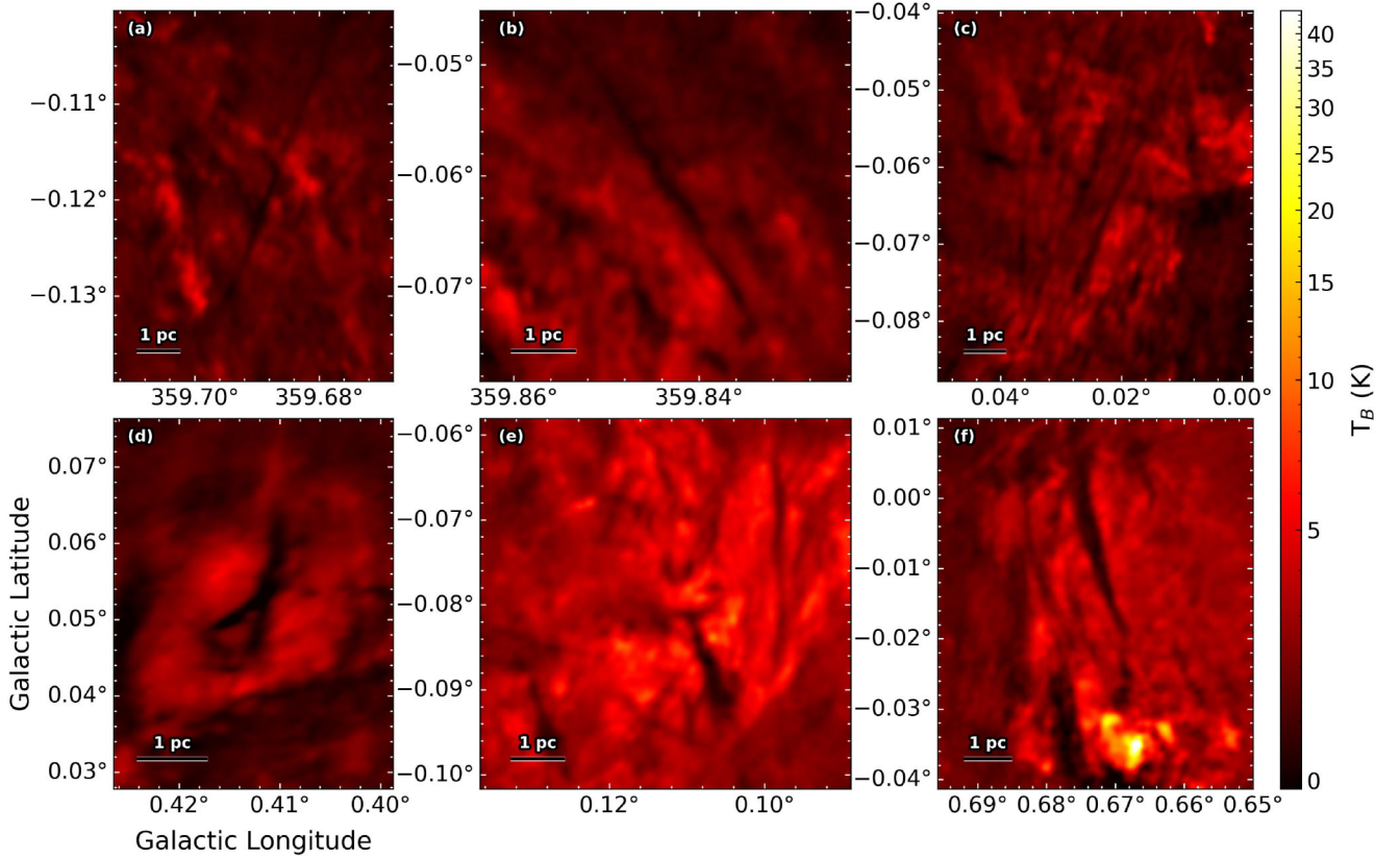
Figure 12. The figure shows examples of the HCO ^+ absorption filaments that are ubiquitous throughout the ACES HCO ^+ data. Each panel shows a single channel from the HCO ^+ cube. (a) G359.689–0.121 (not coincident with named molecular cloud), (b) 20 km s ^{-1} cloud, (c) Sgr A region, (d) dust ridge cloud D, (e) the ‘three little pigs’ complex, and (f) Sgr B2.
