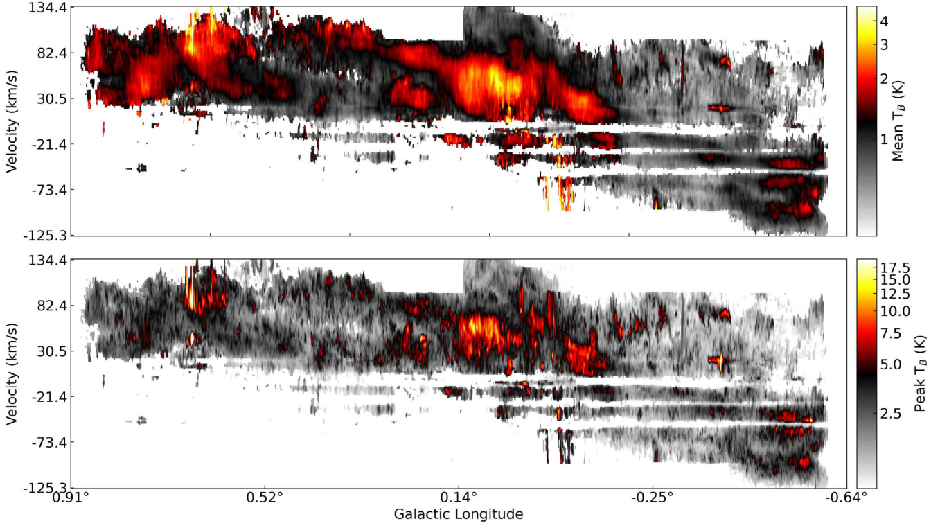
Figure 11. Masked longitude-velocity maps of the HCO ^+ (1–0) emission. The panels show the mean intensity ( top ) and the peak intensity ( bottom ).
