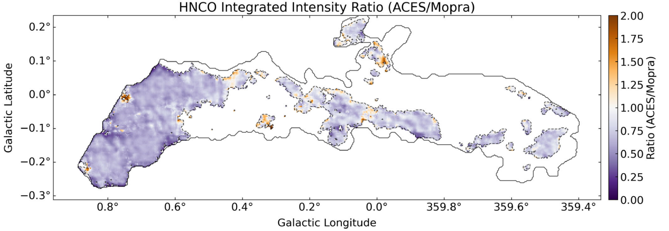
Figure 14. Comparison of the HNC0 (4–3) emission between the Mopra CMZ survey (P. A. Jones et al. 2012) and ACES. The figure shows the ratio map of the ACES HNC0 integrated intensity divided by the Mopra HNC0 integrated intensity. Both cubes were integrated over the same velocity range, and were both masked following the procedure detailed in Section 4.1. The ACES data were reprojected and smoothed prior to the comparison. The solid contour shows the ACES footprint, and the dashed contour shows the footprint of the masked ratio map.
