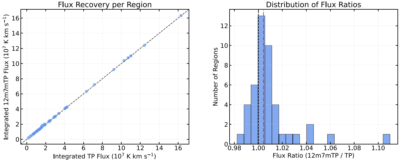
Figure B1. Comparison of the integrated fluxes between the combined 12m7mTP and the TP HNC0 cubes. Integrated fluxes were calculated over a common spatial and spectral extent (Section 3.5.4). The left panel shows a direct comparison of the integrated fluxes, while the right panel shows a histogram of the flux ratios (12m7mTP / TP). In both panels, the dashed black line indicates perfect flux recovery, i.e. a 1-to-1 line in the left figure and a flux ratio of 1 in the right. The red dash-dot line in the right panel shows the median ratio of 1.004.
