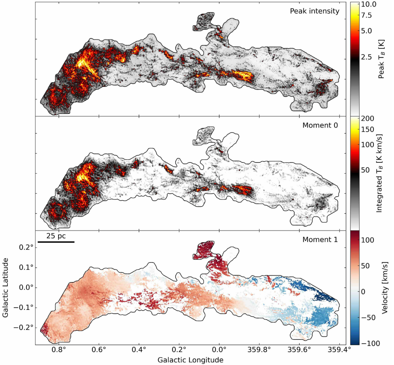
Figure 8. Masked maps of the HNCO (4–3) emission. The panels show the peak intensity ( top ), integrated intensity ( centre ), and the weighted velocity field ( bottom ). The peak intensity and integrated intensity maps are shown on an asinh stretch, while the velocity field is linear. The peak intensity map is masked only using edge masking to suppress elevated noise at field edges. The integrated intensity and velocity maps are masked using the binary dilation method described in Section 4.1, combined with the edge masking. The black contour corresponds to the overall footprint of ACES.
