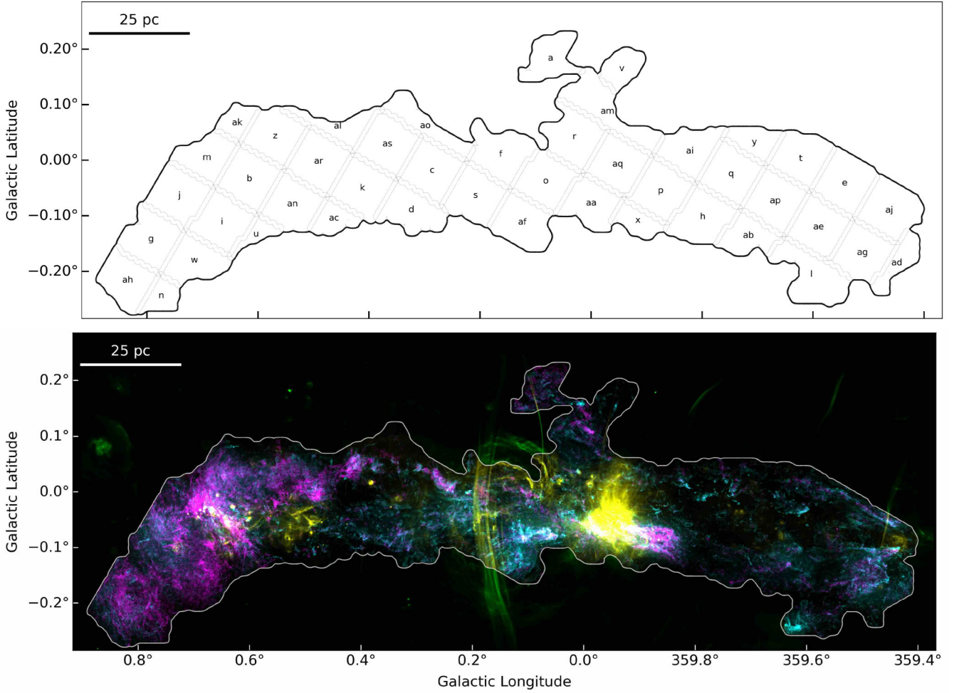
Figure 1. The top panel shows the coverage of ACES. The grey contours show the footprint of the 45 individual ALMA mosaics, where the alphabetical ID in the centre of each corresponds to the field ID (see Section 2 and Tables A2 and A3). The solid black outline shows the overall footprint of ACES resulting from the combination of all 45 mosaics. The bottom panel shows a three-colour image of the CMZ. Magenta: ACES HNC peak intensity (Section 4.1), Cyan: ACES HCO ^+ peak intensity (Section 4.1), Yellow: MeerKAT 1.28 GHz continuum (I. Heywood et al. 2022). The white contour corresponds to the overall footprint of ACES.
