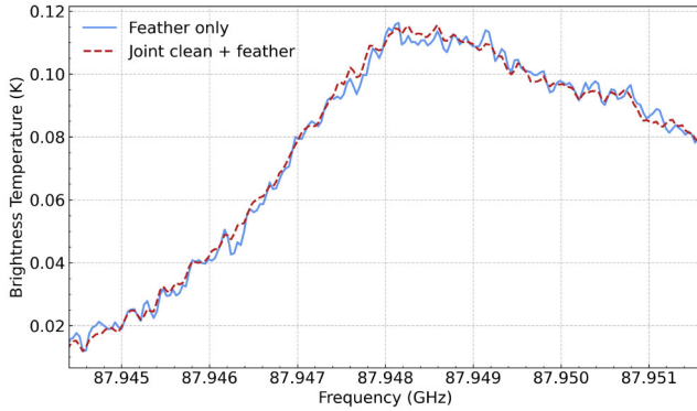
Figure 3. Comparison for field \tau between the two different array combination methods presented in Section 3.5. Shown are the mean spectra for two HNCO cubes, resulting from the different methods. The dashed line shows the mean spectrum of the jointly imaging and feathered cube (Section 3.5.1). The solid line shows the mean spectrum of the feather-only cube (Section 3.5.3). Note that these tests were performed on a small subset of the channels, hence the restricted frequency coverage in the figure.
