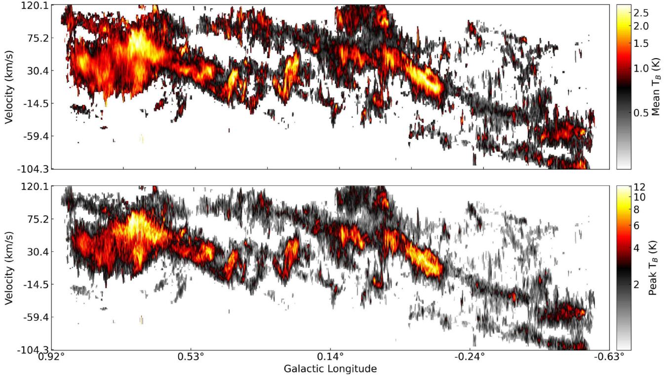
Figure 10. Masked longitude-velocity maps of the HNC(4–3) emission. The panels show the mean intensity ( top ) and the peak intensity ( bottom ).
