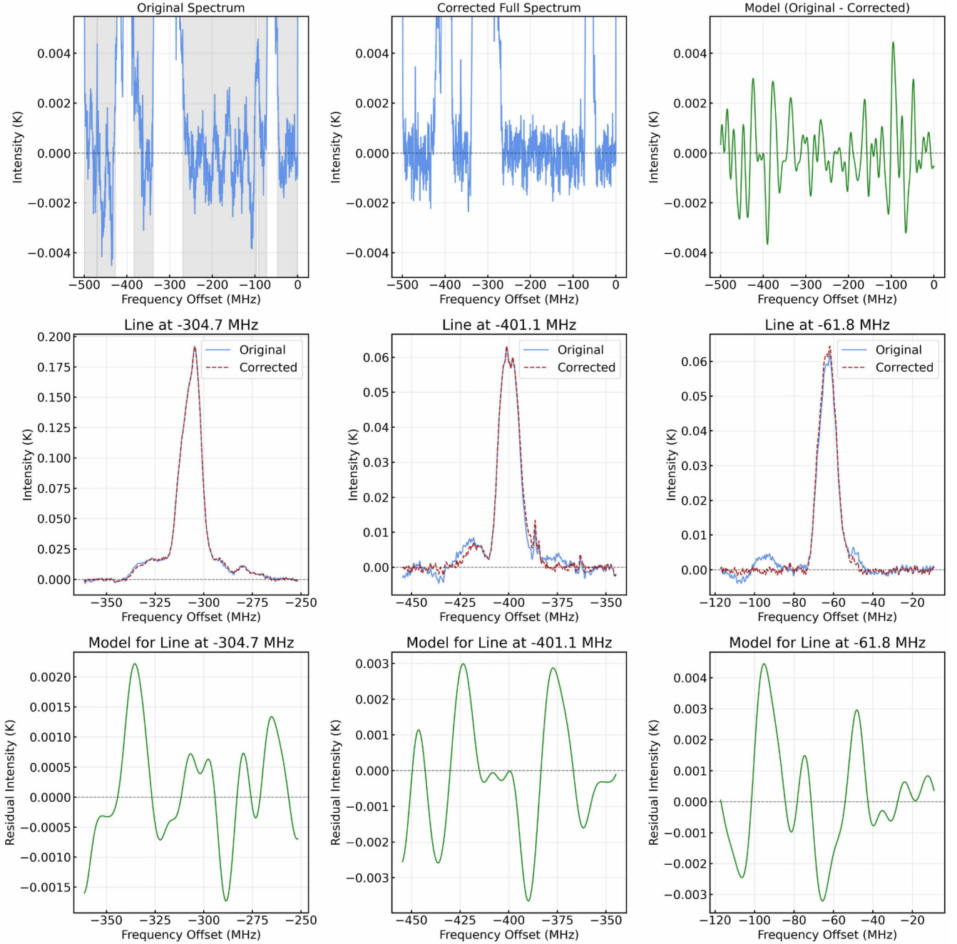
Figure 4. Example showing the Total Power baseline ripple procedure (Section 3.7) for field ak (TP SPW 19). The spectra are taken from the ALMA single-dish pipeline-produced cube, and are spatially averaged across the whole field. Top left: Mean spectrum of the original cube. Shaded regions show the identified line-free channels. Top centre: Corrected mean spectrum after subtracting the model of the baseline ripples. Top right: Model (original - corrected). Note that the y-axes of the panels in the top row have been cropped to highlight the baseline structure. Middle row: the three central panels show zoom-ins of the before (solid line) and after (dashed line) baseline correction spectra for the three most prominent lines. Bottom row: the three bottom panels show the same frequency (x-axis) zoom-ins as the middle row, this time showing the model (original - corrected). In all panels, the dashed horizontal line denotes the zero level for reference.
