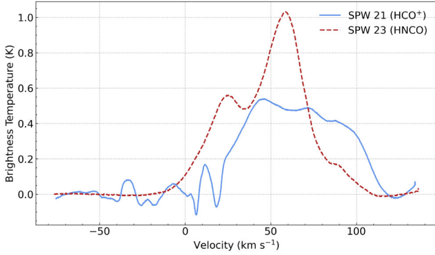
Figure 5. Comparison for field j between the HNCO and HCO + Total Power data. Shown are the mean spectra for each, where the spectra have been spatially averaged across the full field.
