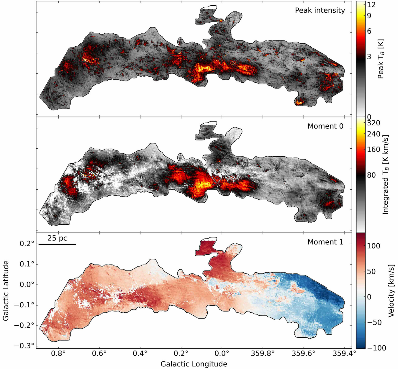
Figure 9. Masked maps of the HCO + (1–0) emission. The panels show the peak intensity ( top ), integrated intensity ( centre ), and the weighted velocity field ( bottom ). The peak intensity and integrated intensity maps are shown on an asinh stretch, while the velocity field is linear. The peak intensity map is masked only using edge masking to suppress elevated noise at field edges. The integrated intensity and velocity maps are masked using the binary dilation method described in Section 4.1, combined with the edge masking. The black contour corresponds to the overall footprint of ACES.
