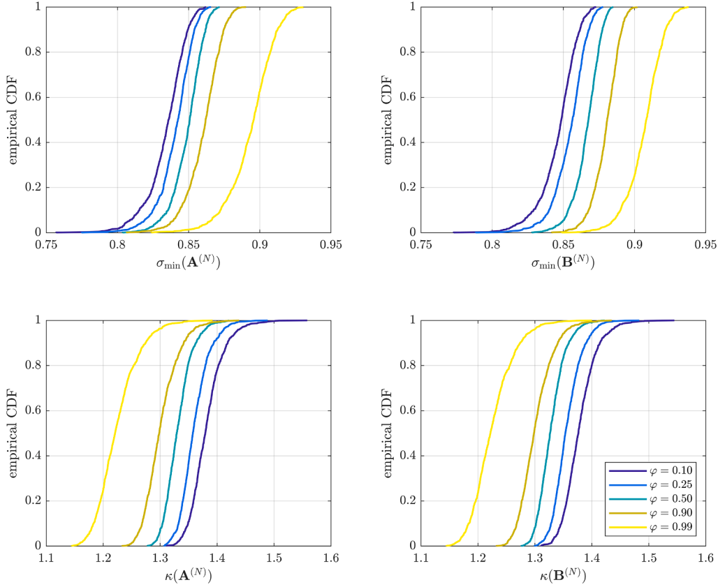
Fig. 3. Empirical cumulative distribution functions obtained via Monte Carlo.
