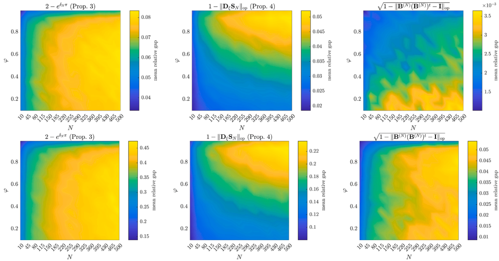
Fig. 4. MRG of the different lower bounds obtained in Section 3.
