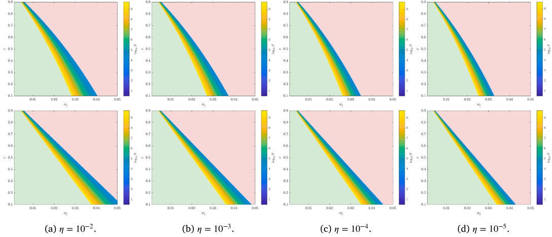
Fig. 2. Contour plots of the right-hand side of (13) (first row) and (19) (second row) as functions of \sigma_\epsilon and \epsilon . In the pink region the bound falls below 10^3 , while in the light green region it exceeds 10^{10} . We remark that, in ADC applications, \sigma_\epsilon represents the average deviation from the ideal sampling instants nT_s , so that \sigma_\epsilon \ll T_s and \sigma_\epsilon/T_s is typically of the order of 1% or less. Higher values of \sigma_\epsilon may correspond to harsher scenarios, but more likely reflect poor hardware designs.
