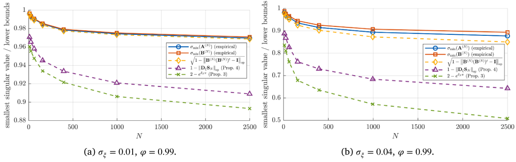
Fig. 1. The figures above show that the obtained bounds are loose.
