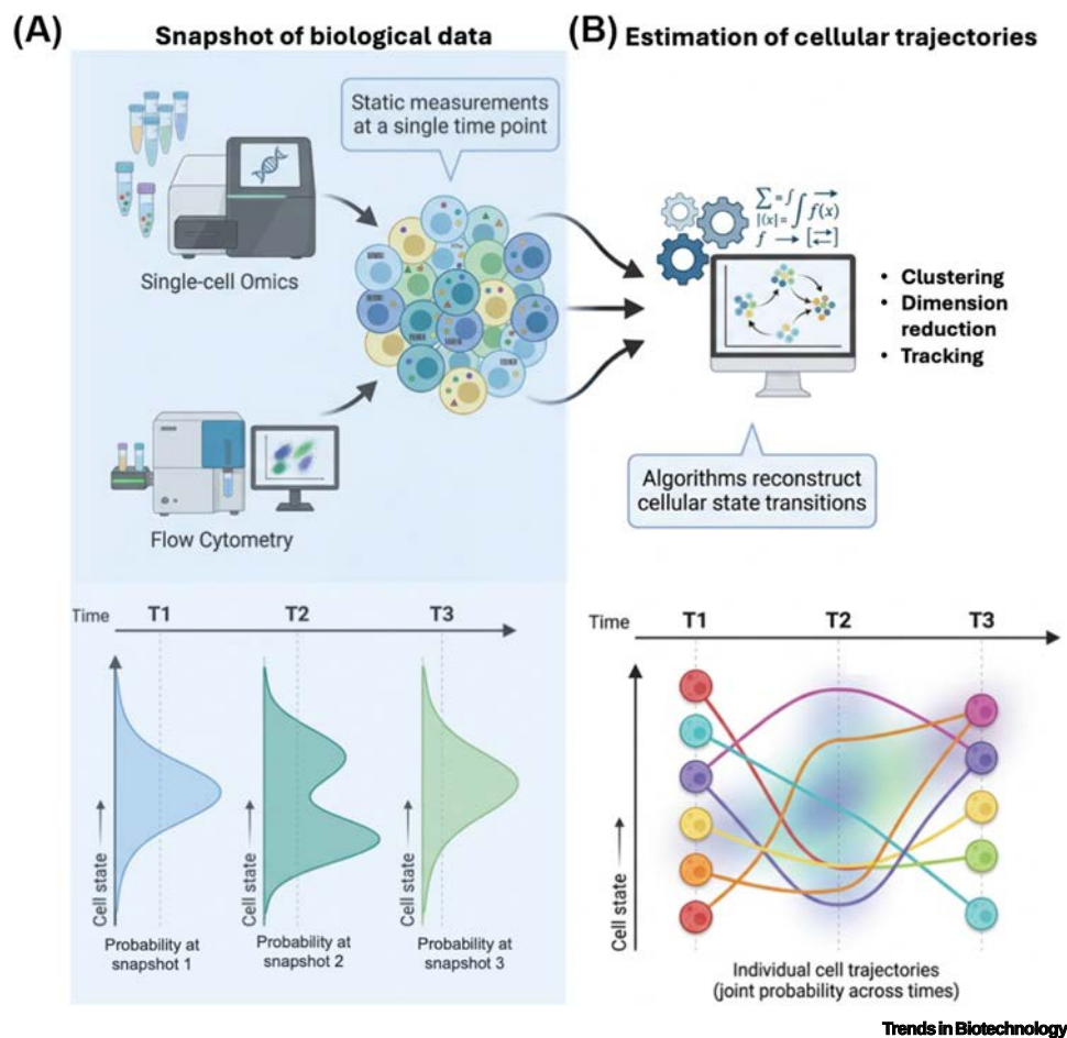
Figure 2. From single-cell snapshots to cellular trajectories: the challenge of reconstructing SP dynamics. (A) Snapshot measurements capture the marginal distribution of cell states at a single time point. Single-cell omics and flow cytometry generate measurements of heterogeneous cell populations, resolving distinct SPs (represented by differently colored and shaped cells). When collected at successive time points (T1, T2, and T3), each measurement provides only the snapshot of cell states at that instant, a series of disconnected cross-sections that does not directly reveal how individual cells or SPs transition between states over time. (B) Computational approaches reconstruct cellular trajectories from snapshot data. Applying dimensionality reduction, clustering, and trajectory inference algorithms to the snapshot data allows the reconstruction of cellular state transitions. As individual cells cannot be tracked continuously over time, the resulting trajectories represent slices of the probability distribution of cell states at various times, posing what is often an ill-posed inference problem whose solution depends on the constraints and assumptions built into the algorithm. Colored lines depict individual paths that cell SPs can take from T1 to T2 and then to T3, illustrating the diversity of possible transition paths between SPs. SPs: subpopulations.
