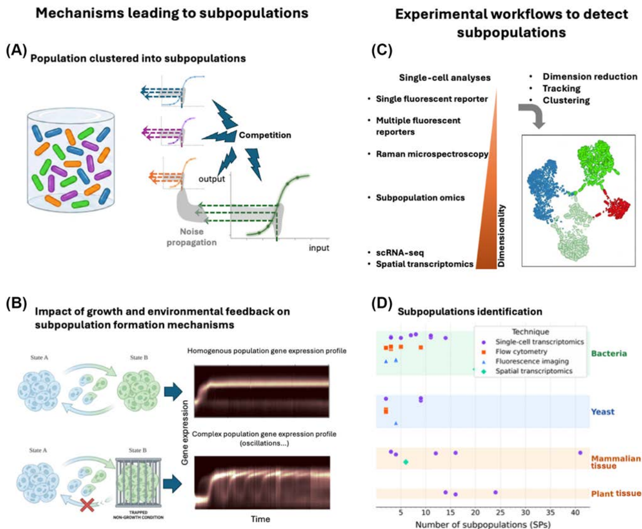
Figure 1. Mechanisms generating cellular subpopulations and experimental strategies for their detection. (A) Biological noise broadens the distribution of cellular responses to a given input, converting a homogeneous population into a phenotypically heterogeneous one. Noise propagation across regulatory networks and competitive interactions between cell types drive the organization of the population into discrete SPs, each following distinct trajectories of gene expression and biological function. (B) Growth feedback on gene expression adds another layer of complexity to cell population dynamics. (C) Experimental workflows for SP detection span increasing levels of dimensionality, from single fluorescent reporters and multiplexed biosensor panels to single-cell RNA-sequencing (scRNA-seq). Dimensionality reduction, temporal tracking, and clustering convert high-dimensional data into an interpretable SP map. (D) The application of various single-cell approaches to diverse biological systems has led to the discovery of a limited number of SPs (links to references and experimental details are provided in Table 1). SPs: subpopulations.
