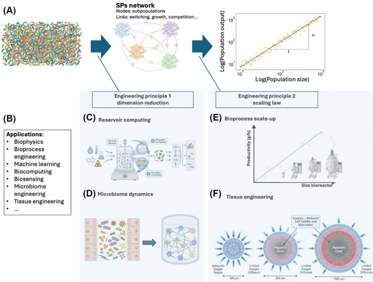
Figure 3. Emergence of new engineering principles from SP networks. (A) Left: a cell population that appears highly complex at the individual level, with each cell tracing its own trajectory through a vast phenotypic space driven by stochastic gene expression, metabolism, and cell cycle progression, self-organizes into a discrete set of functionally distinct SPs. Nodes represent SPs and directed, weighted edges encode rates of phenotypic switching and competitive or cooperative interactions between them, forming an SP network. (A) Center: this self-organization collapses the high-dimensional phenotypic space onto a low-dimensional manifold. Despite the thousands of molecular variables involved, the collective behavior of the population can be captured and controlled by a small number of emergent coordinates, represented here as a compressed low-dimensional state space. This dimensionality reduction is a general property of populations organized into SP networks, independent of the specific biological system considered. (A) Right: once collective dynamics operate on a low-dimensional manifold, scaling laws of the form P \sim N^\alpha become accessible, where P is a measure of collective performance and N is population or system size. When \alpha is greater than one, the system exhibits superlinear scaling, producing disproportionately greater output as it grows, a signature of collective efficiency arising from optimized interaction structure. The log-log linearity of this relationship, with slope greater than one, is the fingerprint of low-dimensional manifold dynamics. (B–F) Four applications illustrate the generality of these two principles across scientific fields: (C) reservoir computing, where microbial consortia provide naturally rich, heterogeneous, and memory-bearing dynamical responses that satisfy the computational requirements of a high-quality reservoir; (D) microbiome engineering, where SP-aware niche design and biosensor interpretation enable more accurate characterization and control of community function; (E) bioprocess scale-up, where SP network structure governs the trade-off between growth and production and may yield principled scale-up rules; and (F) tissue engineering, where oxygen transport scaling laws and dimensionality reduction of cell state dynamics together constrain and guide construct design across scales.
