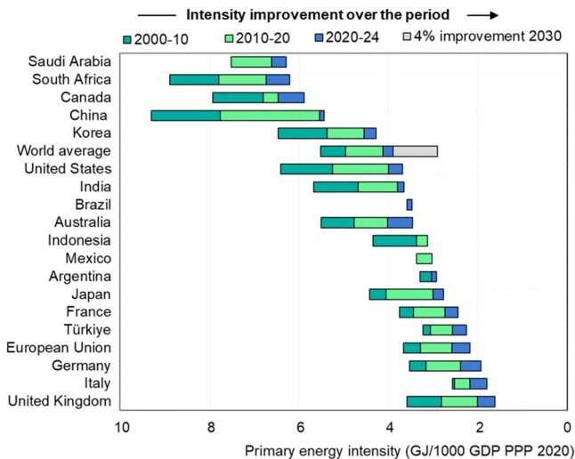
Figure 4 Energy intensity improvements for selected countries and regions. Source: IEA, World Energy Indicators, 2026. Note: 4% improvement 2030 = actuals to 2024 and 4% per year on average to 2030 consistent with the IEA Net Zero Emissions by 2050 Scenario.
